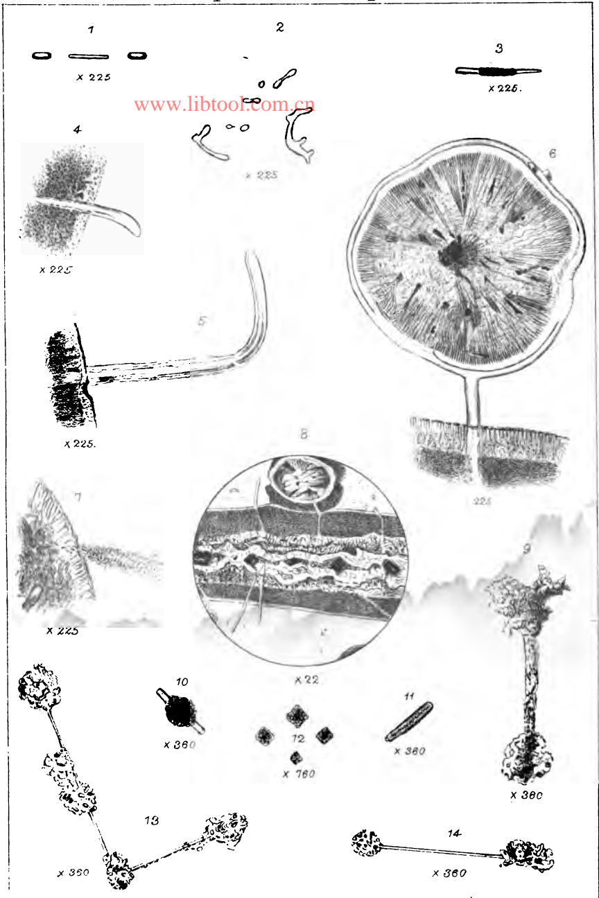
Structures in Obsidian and Leucite.
