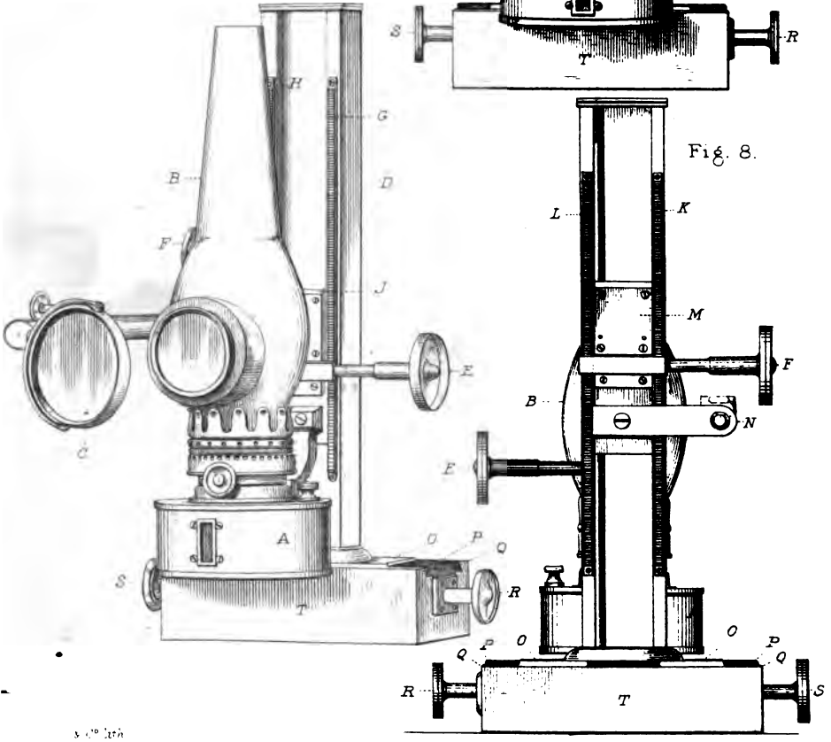
M r Dallinger's new microscope lamp.
