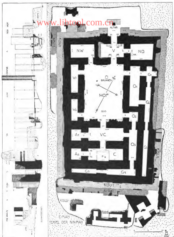
FIG. 38.—Ground-plan and section of Ninmach Temple.
