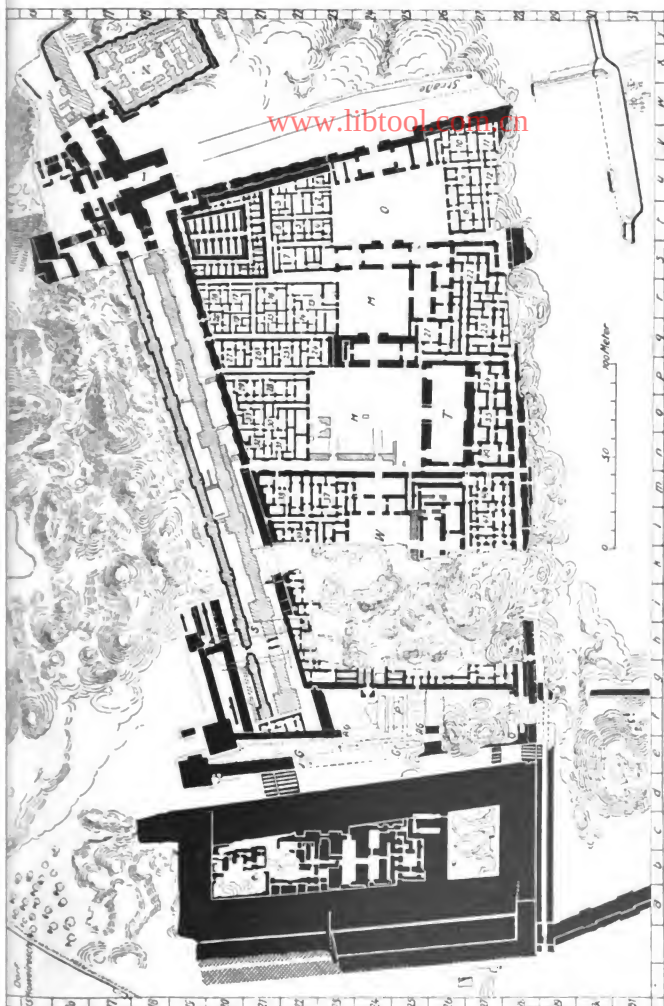
FIG. 44.—Complete plan of Southern Citadel. N. Ninnach Temple. I. Ishar Door.
