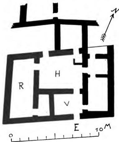
FIG. 241.—Ground-plan of house in Fara (Shuruppak).
