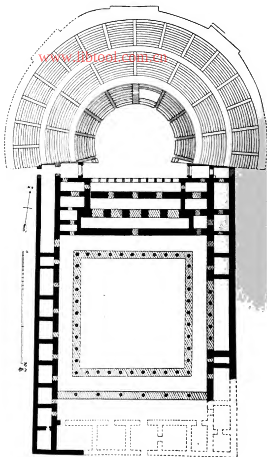
FIG. 253.—Plan of Greek theatre, restored.
