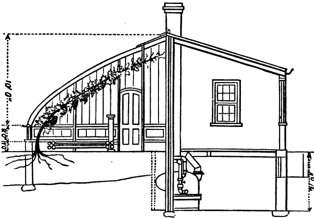
Fig. 63.—SECTION OF FORCING GRAPERY.
