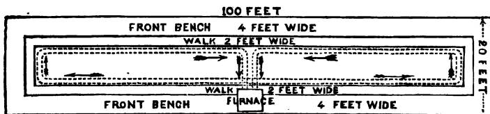
FIG. 42.—PLAN OF GREENHOUSE HEATED BY DOUBLE FLUES.
