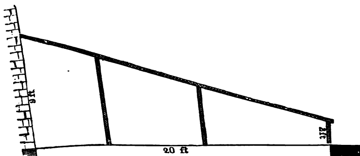
Fig. 60.—LEAN-TO GRAPERY.
