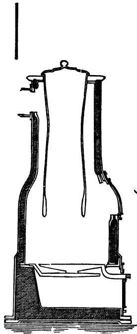
Fig. 37.—SECTION.
