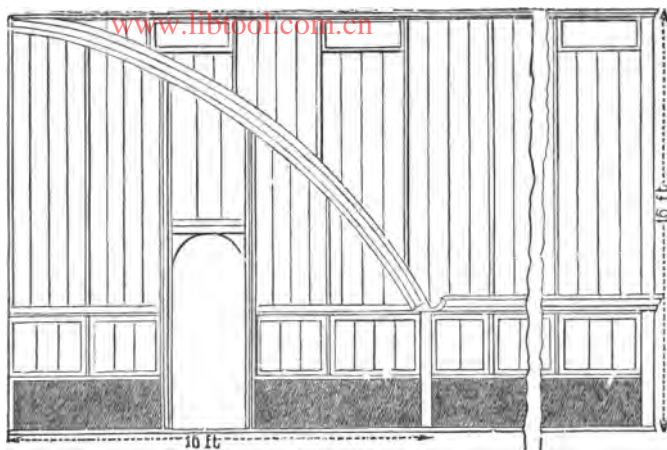
Fig. 38.—ELEVATION OF CONSERVATORY ATTACHED TO DWELLING.
