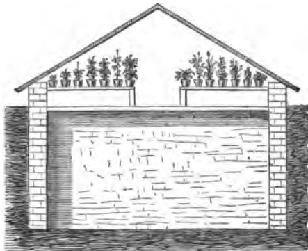
Fig. 47.—GREENHOUSE AND CELLAR COMBINED.
