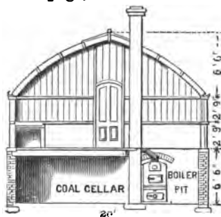
Fig. 44.—END-VIEW OF FIG. 43, AT BOILER PIT.
