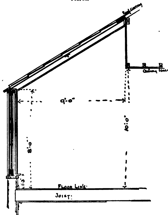
SECTION OF SKYLIGHT
