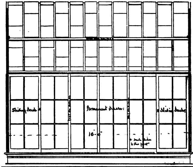
ELEVATION of SKYLIGHT: from inside
