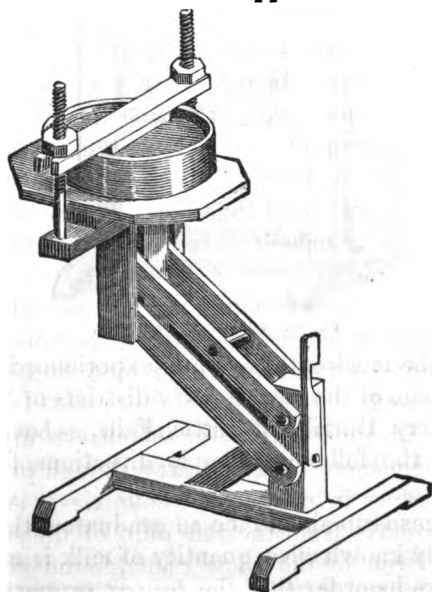
Fig. 82. Cheese-press.
