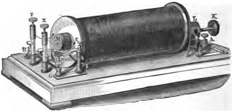
Fig. 40.—The Induction-Coil.
