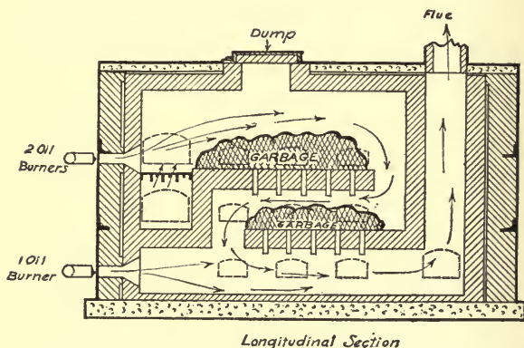
FIG. 25.—Morse-Boulger destructor, longitudinal section.
