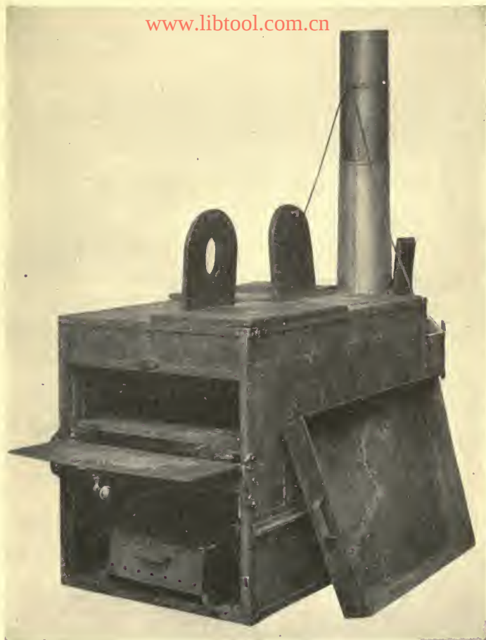
FIG. 29.—Incinerator for excreta, Quartermaster Corps type.
