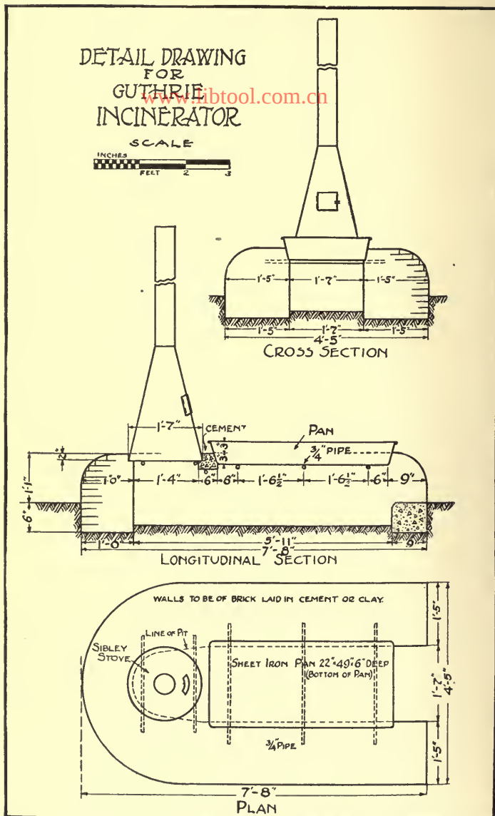
FIG. 36.—Guthrie incinerator, for disposal of garbage, solid and liquid.
