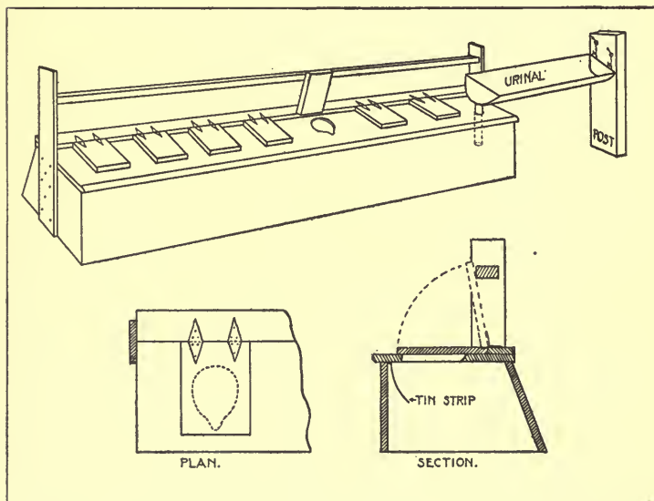
FIG. 32.—Box seat cover and urine trough for company sink. Note shape of seat, self-closing cover, slope of back, and tin strip (after Straub and Miller).
