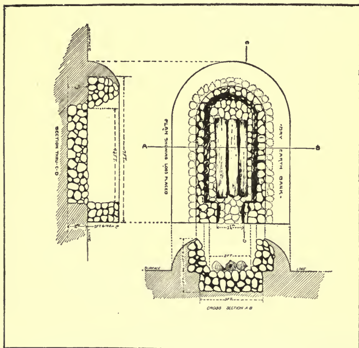
FIG. 35.—Company mess incinerator ( Straub )
