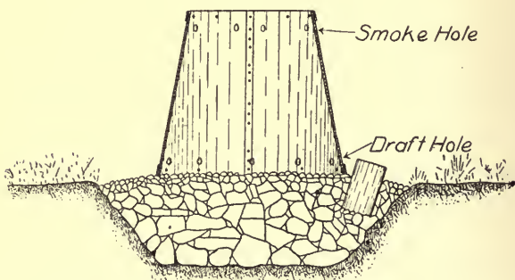
Central Section of Incinerator and Pit
