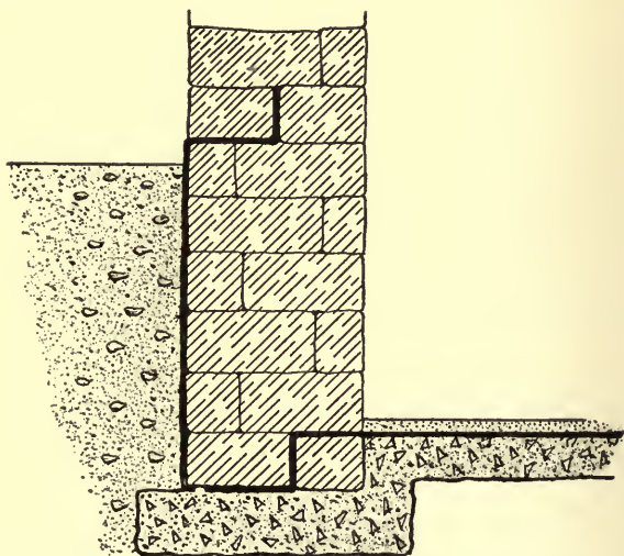
FIG. 40.—Damp-proof course for foundations of buildings (indicated by the heavy line).
