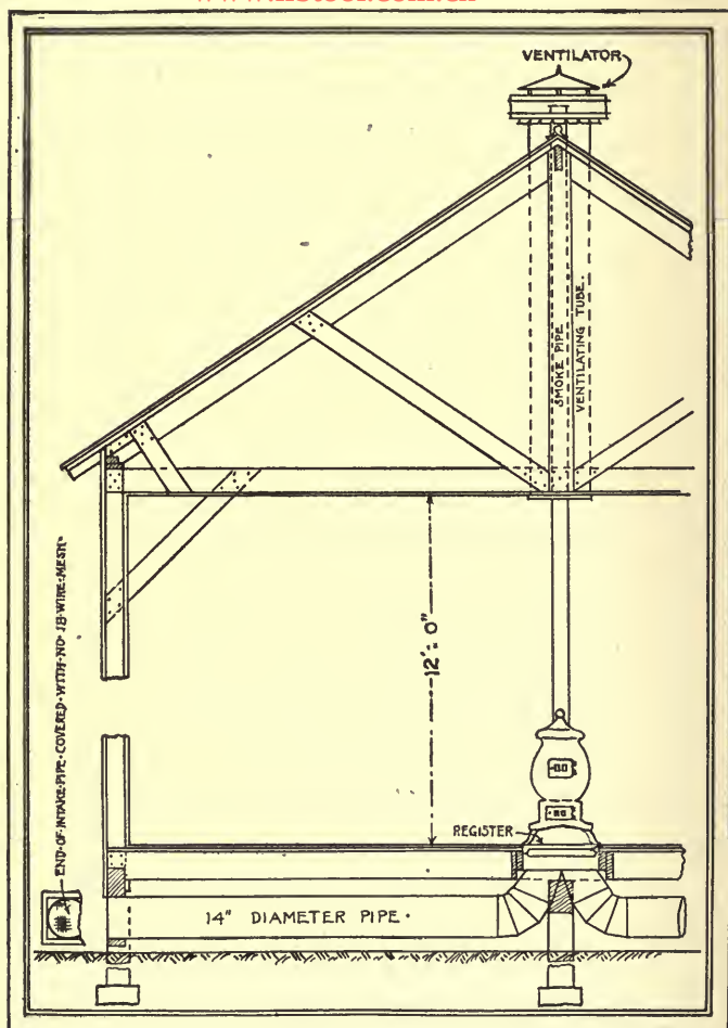
FIG. 43.—Ventilation system for temporary buildings by means of fresh-air ducts beneath floors, opening under stoves.
