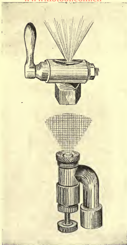
FIG. 47.—Above, Bordeaux nozzle for spraying oils. Below, Vermorel nozzle for spraying watery solutions.
