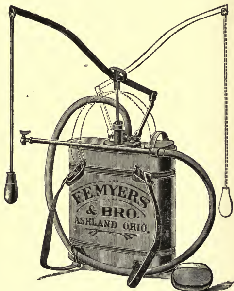
FIG. 46.—“Knapsack” spray pump for oiling standing water.
