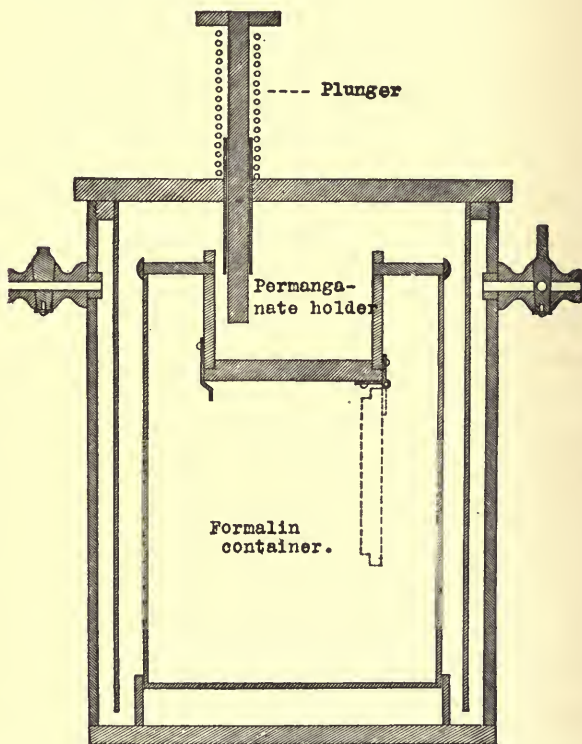
FIG. 52.—Gas generator, for disinfection in the field. Height, 8 inches; diameter, 6 inches; weight, 5 pounds.
