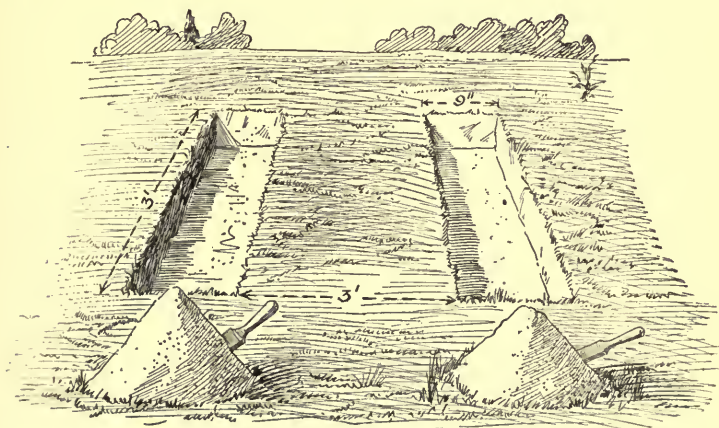
FIG. 34.—Shallow “straddle” trenches for excreta.
