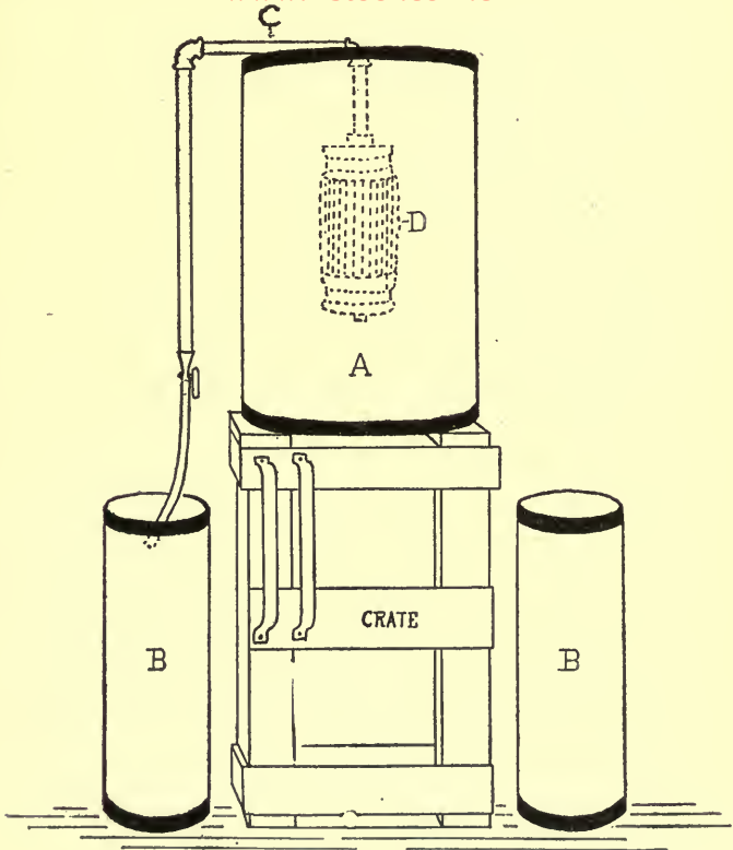
FIG. 19.—Darnall filter, showing method of operation.
