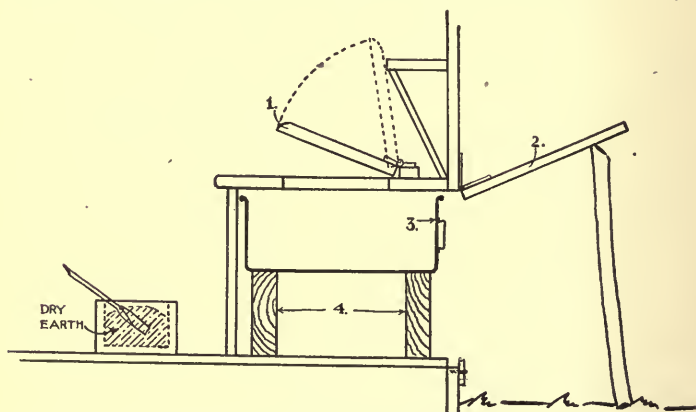
FIG. 22.—Dry earth closet: 1, Self-closing seat cover; 2, fly-tight trapdoor; 3, pan; 4, supports for pan.
