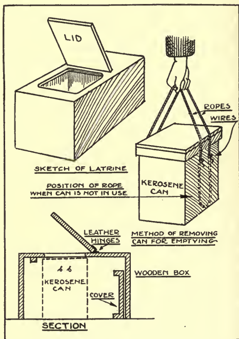
FIG. 54.—Improved latrine bucket, seat and cover, for use in trenches (after Lelean).
