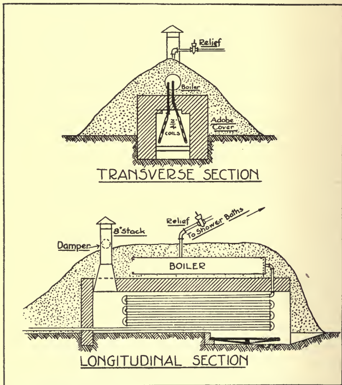
FIG. 50.—Saville bath-water heater (after Lewis and Miller).
