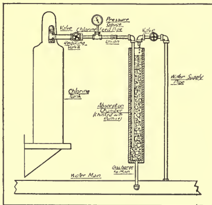
FIG. 16.—Simple apparatus for sterilization of water by chlorine gas.
