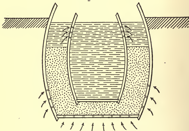
FIG. 20.—Barrel filter sunk in spring.
