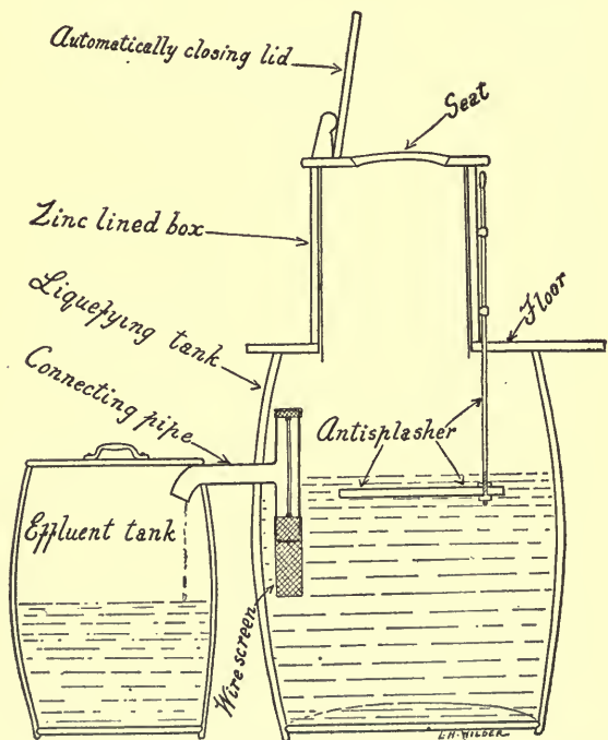
FIG. 23.—Closet devised by officers of the United States Public Health Service (Lumsden, Roberts, and Stiles).
