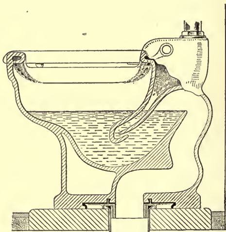
FIG. 44.—Siphon jet closet, "West Point" model ( J. L. Mott Co. ).
