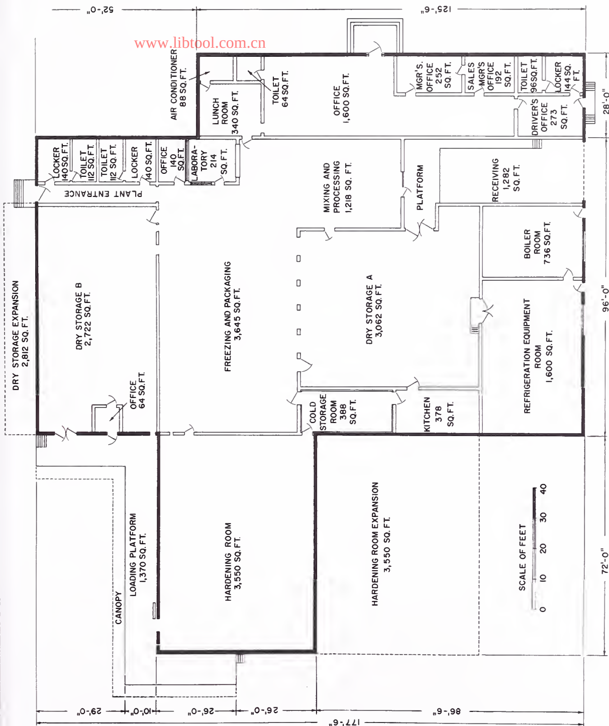
FIGURE 5.—Suggested layout for an automated plant manufacturing 1 million gallons of ice cream and 250,000 gallons of novelties annually.
