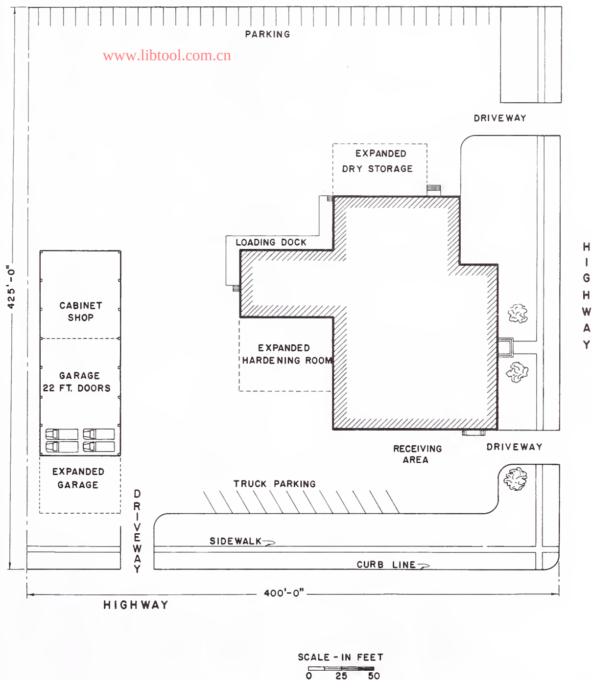
FIGURE 7.—Suggested layout for the site of an automated ice cream plant manufacturing 1\frac{1}{4} million gallons of ice cream and novelties annually.
