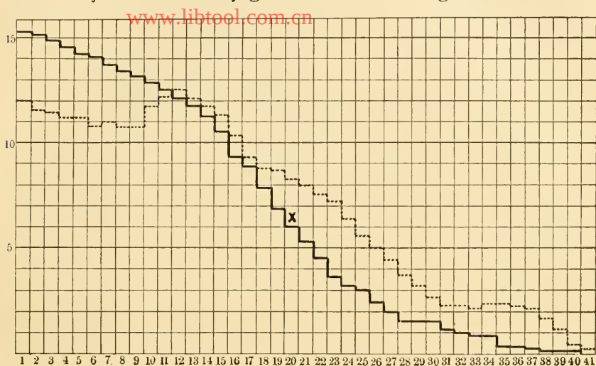
Fig. 64—A VITALITY CURVE OF UROLEPTUS MOBILIS
