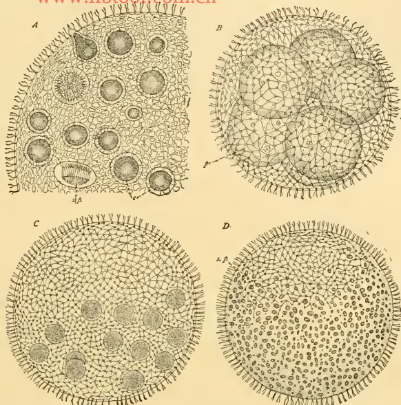
Fig. 26—TYPES OF VOLVOX COLONIES
