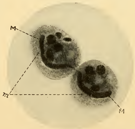
Fig. 49—EUPLOTES' PATELLA IN DIVISION
