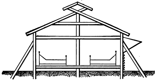
Portable hut. From Notter and Firth's Hygiene (By the courtesy of Messrs. F. Blackiston & Co.)
