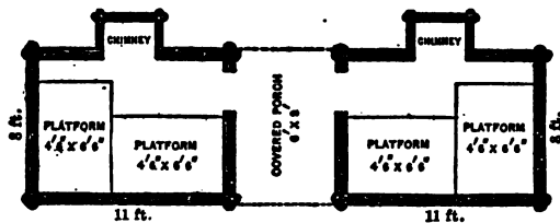
Ground Plan of Squad Huts for Four, each with Covered Porch.
