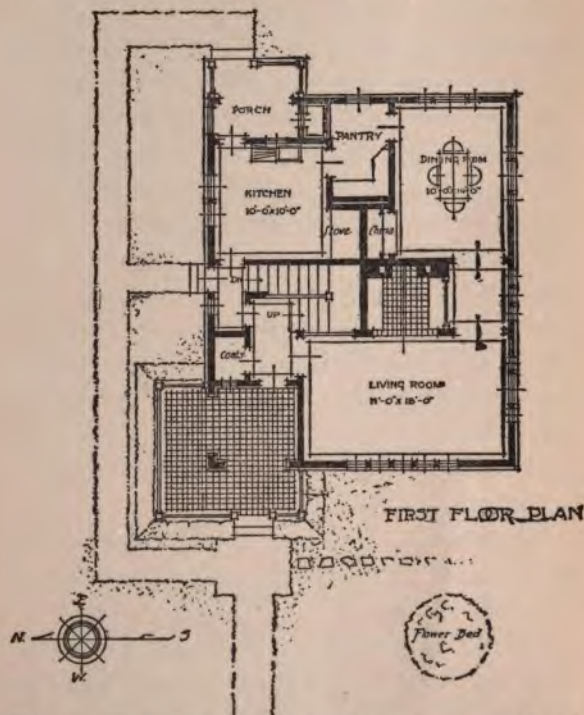
Fig. 11. First Floor Plan of a $5,000 house, by C. M. Craig, Architect.
