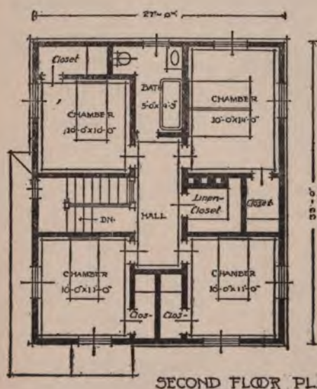
Fig. 12. Second Floor Plan of the Craig house.
