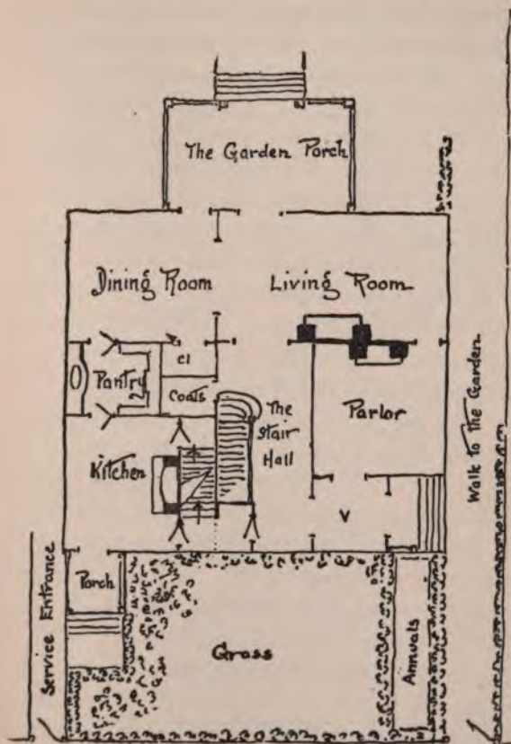
Fig. 17. Fifty-foot lot, plan of the ground floor.
