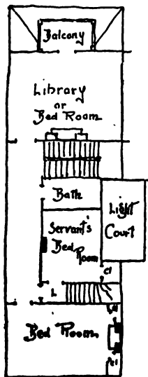
Fig. 23. Plan of the Second Floor (third floor similar).
