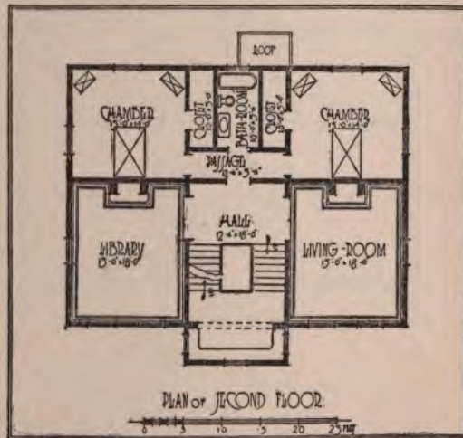
Fig. 10. Second Floor Plan of an Austrian house.
