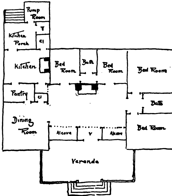
Fig. 20. Plan of a Bungalow, second stage.
