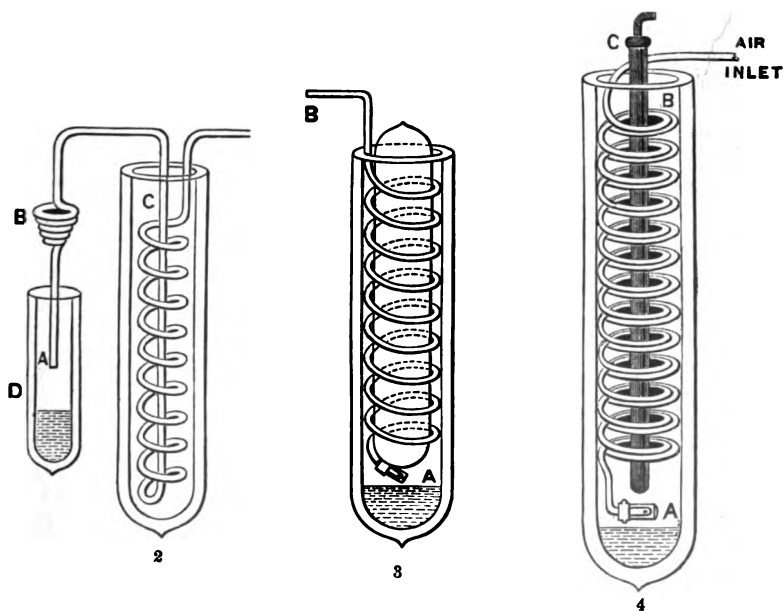
2, 3, 4. DIFFERENT ARRANGEMENTS OF REGENERATING COILS.
