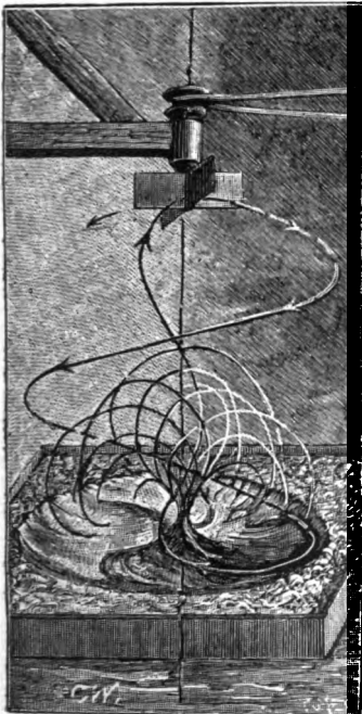
PHYSICAL PHENOMENA OF UPPER ATMOSPHERE.
