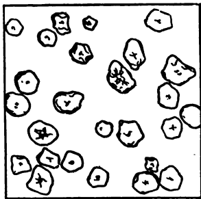
FIG. 17.—Maize Starch.
