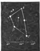
Cephalopoda (in oberer Rulmination).
