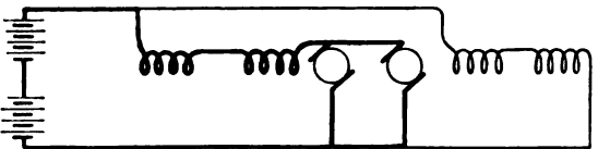
KRIEGER SYSTEM OF SPEED-REGULATION.
