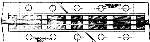
PLAN OF RAIL-JOINT; HULL TRAMWAYS.
