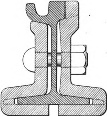
SECTION OF JOINT USED AT PORTSMOUTH
