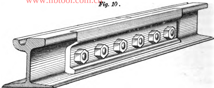
"DICKER" JOINT.
