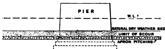
RUBBLE APRON TO PIERS.
