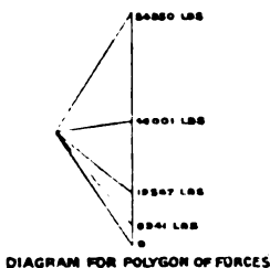
DIAGRAM FOR POLYGON OF FORCES
