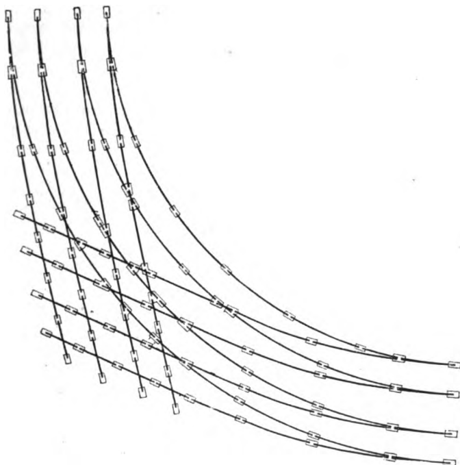
PLAN OF SPECIAL TRACK-WORK AT FITZALAN SQUARE, SHEFFIELD.
