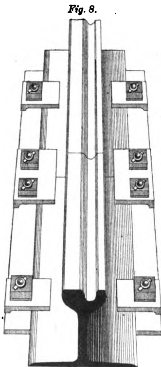
MARSHALL JOINT - PLATES
