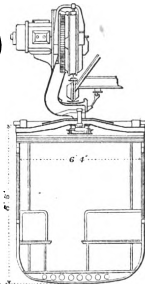
SECTION OF BOGIE FRAME AND CARRIAGE SHOWING MODE OF SUSPENSION
