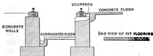
CROSS-SECTION OF RUNNING-SHED PIT.
