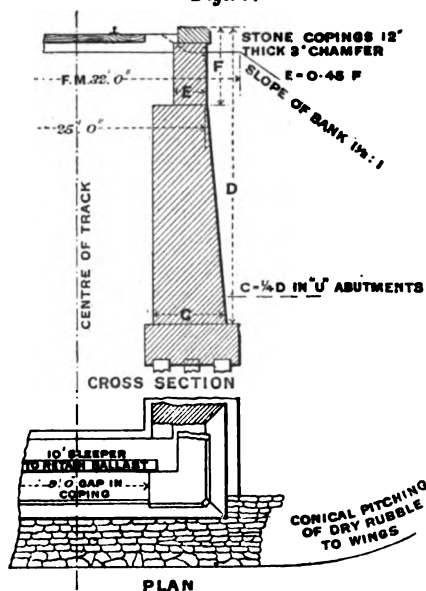
DIAGRAMS OF CONCRETE WING-WALL.
