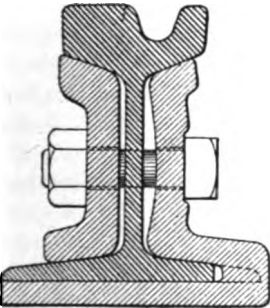
PHOENIX JOINT
