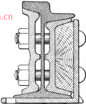
WEBER JOINT
