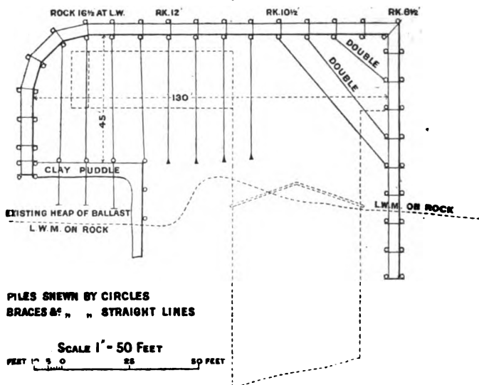
PLAN OF COFFER-DAM.
