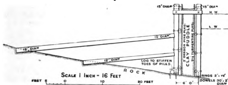
CROSS-SECTION OF COFFER-DAM.
