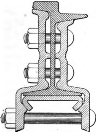
CHURCHILL JOINT
