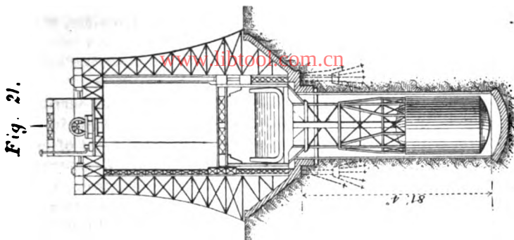
SECTIONAL ELEVATION OF CANAL-LIFT SHOWING SCREW SPINDLE AND FLOAT IN WELL.
