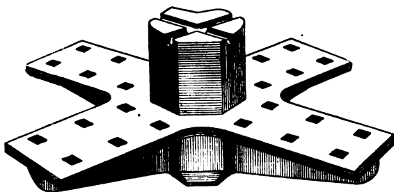
SOLE-PLATE CROSSING.
