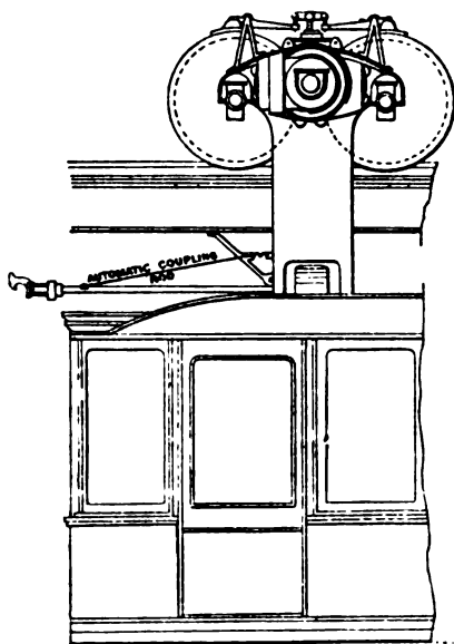
ELEVATION OF BOGIE AND END OF CARRIAGE
