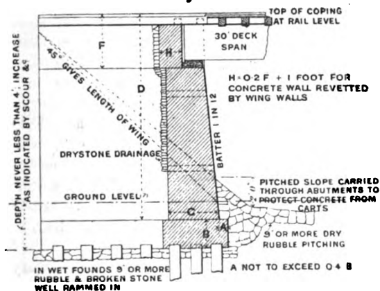
DIAGRAM OF CONCRETE ABUTMENT.
