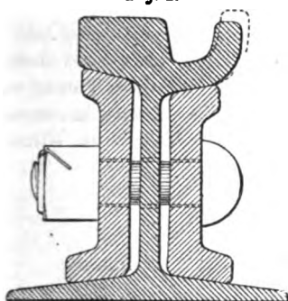
SECTION OF RAIL AND FISHPLATES
