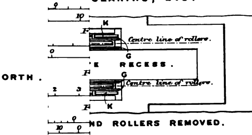
Fig. 2. GEARING, ETC.
