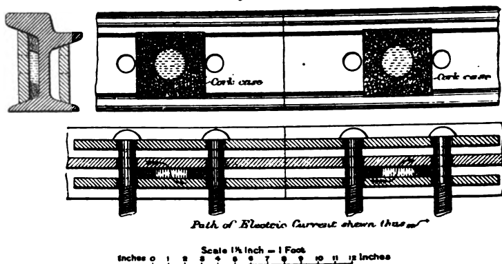
EDISON-BROWN RAIL-BOND.
