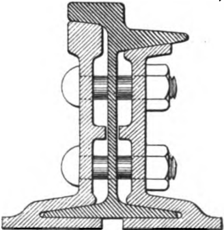
CONTINUOUS - RAIL JOINT
