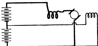
JEANTAUD SYSTEM OF SPEED-REGULATION.
