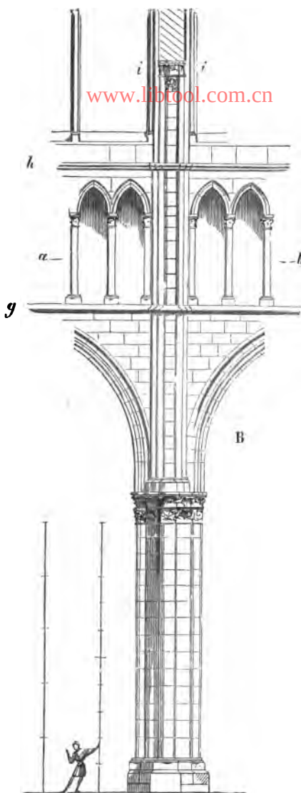
FIG. 36.—PIERS AND SUPERSTRUCTURE, RHEIMS CATHEDRAL. (1211-1240.)
