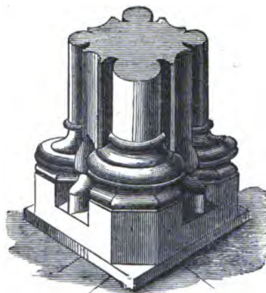
FIG. 4.—BASE OF DECORATED SHAFT.
