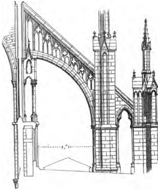
FIG. 2.—FLYING BUTTRESS.
