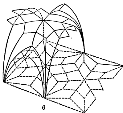
FIG. 99.—VAULTS.
