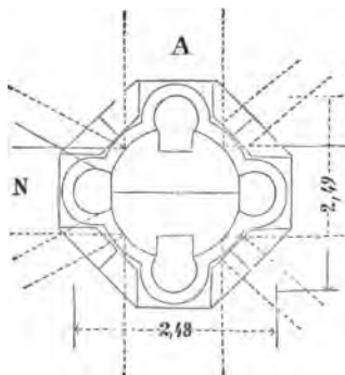
FIG. 36.—PIERS AND SUPERSTRUCTURE, RHEIMS CATHEDRAL. (1211-1240.)
