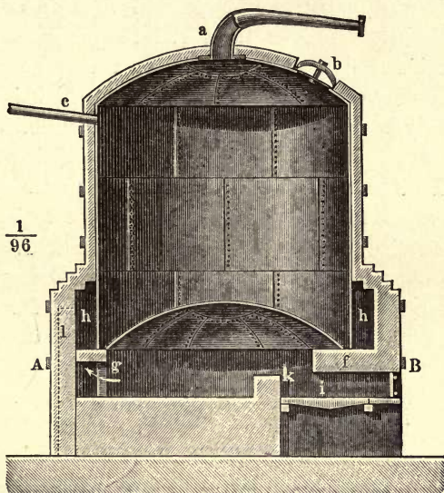
FIG. 6.—Sectional diagram of tar-still with arched bottom. The fire-place is at i ; the hot gases pass over the bridge k and through g into the flues h, h . The pipe at c is to supply the still with tar ; a is the exit pipe connected with the condenser, and b a man-hole for cleaning out the still. The condenser and bottom pipe for drawing off pitch have been omitted to avoid complication.
