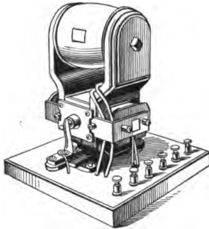
FIG. 142.—MAGNETO-GENERATOR FOR DEVELOPING A SINUSOIDAL CURRENT.
