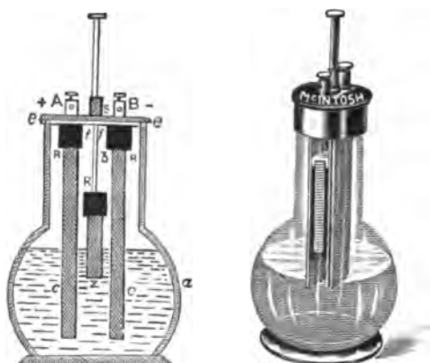
FIG. 27.—GRENET CELL.
