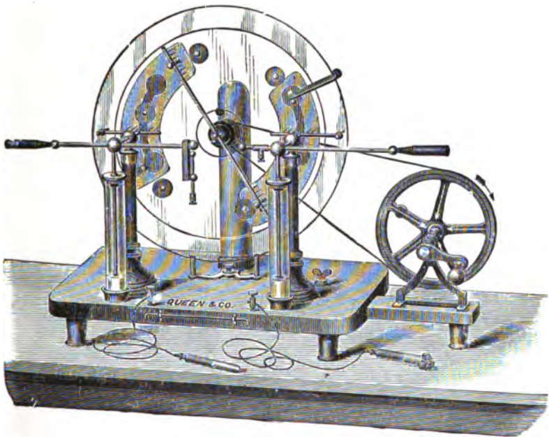
FIG. 13.—HOLTZ MACHINE.
