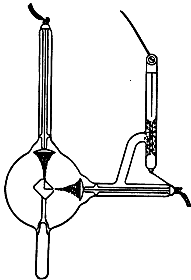
FIG. 154.—AUTOMATIC ADJUSTABLE VACUUM X-RAY TUBE, FOR USE WITH ALTERNATING CURRENTS.
