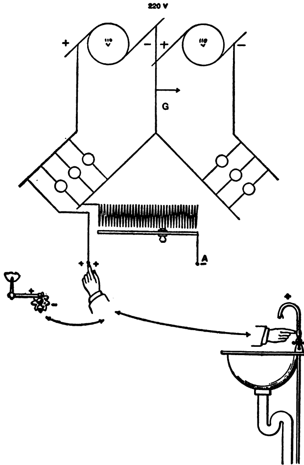
FIG. 135.—DIAGRAM SHOWING THE DANGER OF THE THREE-WIRE SYSTEM.
