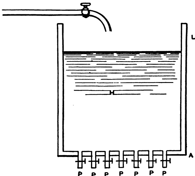
FIG. 60.—SHOWING THE RELATION OF PRESSURE TO OUTFLOW IN A WATER TANK.
