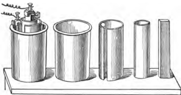
FIG. 26.—BUNSEN CELL AND ITS COMPONENT PARTS.
