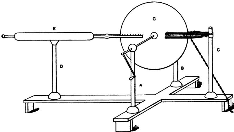
FIG. 9.—SIMPLE GLASS PLATE MACHINE.
