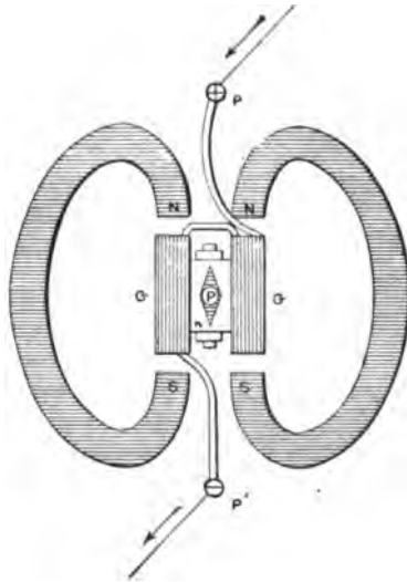
FIG. 57.—SHOWING HOW THE AMMETER NEEDLE IS MOUNTED.
