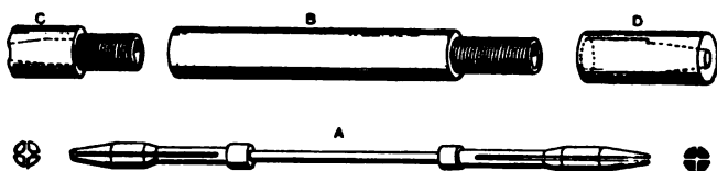
FIG. 127.—COMBINATION ELECTRODE HANDLE.
