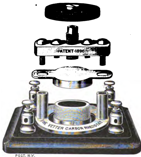
FIG. 110.—WORKING PARTS OF VETTER RHEOSTAT.
