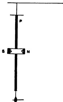
FIG. 56 A.—ARRANGEMENT OF AMMETER NEEDLE.
