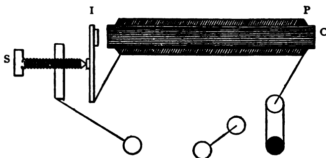
FIG. 139.—SHOWING CIRCUIT BREAKER AND ITS CONNECTIONS.
