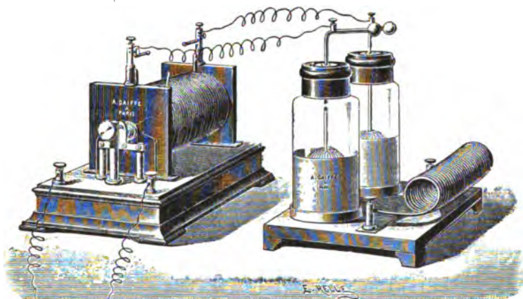
FIG. 144.—APPARATUS FOR OBTAINING A HIGH FREQUENCY CURRENT.
