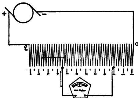
FIG. 113.—SHOWING METHOD OF REGULATION OF CURRENT BY PLACING RESISTANCE IN CIRCUIT.
