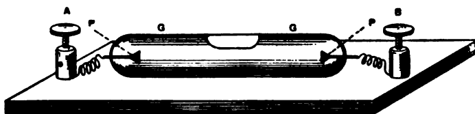
FIG. 132.—POLE TESTER.
