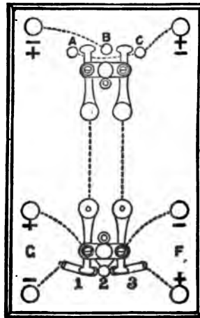
FIG. 117.—GALVANO-FARADAIC COMBINER.
