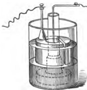
FIG. 24.—GRAVITY CELL.
