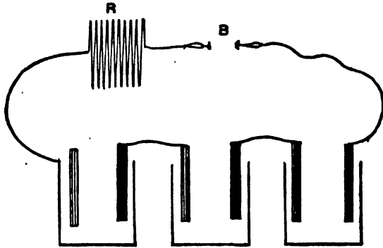
FIG. 114.—SHOWING A RHEOSTAT PLACED IN CIRCUIT.
