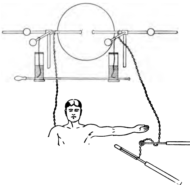
FIG. 95.—METHOD OF APPLYING THE LEYDEN JAR SPARK.
