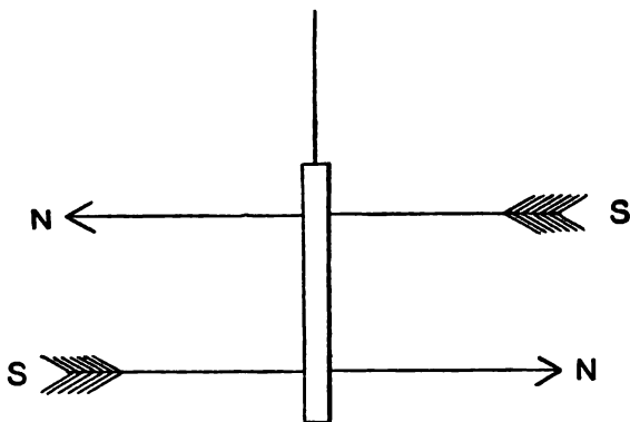
FIG. 50.—AN ASTATIC SYSTEM OF NEEDLES.
