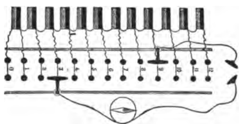
FIG. 104.—GAIFFE'S CELL SELECTOR.
