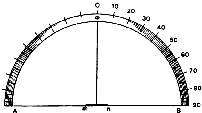
FIG. 53.—SCALE OF MIRROR GALVANOMETER.
