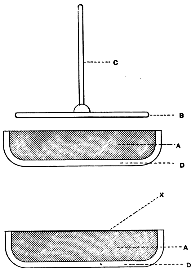
FIG. 12.—THE ELECTROPHORUS.
