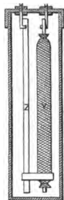
FIG. 32.—SILVER CHLORID CELL.
