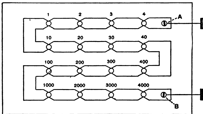
FIG. 63.—ARRANGEMENT OF RESISTANCE COILS.
