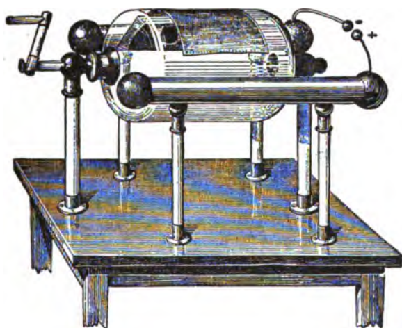
FIG. 11.—CYLINDER MACHINE.
