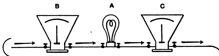
FIG. 66.—SHOWING THE METHOD OF DETERMINING UNKNOWN RESISTANCES BY MEANS OF AN AMPÈRE METER AND A VOLT METER.
