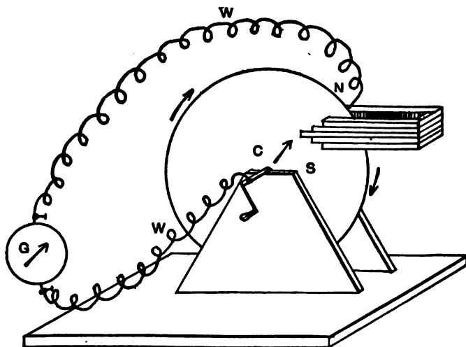
FIG. 69.—FARADAY'S MAGNETO-ELECTRIC MACHINE.
