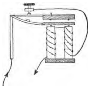
FIG. 140.—THE NEEF OR WAGNER HAMMER.
