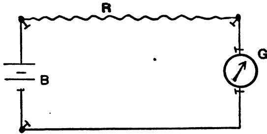
FIG. 36.—SHOWING A SIMPLE CIRCUIT CONTAINING ONE RESISTANCE WIRE.
