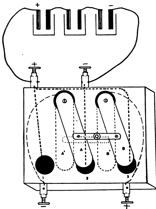
FIG. 116.—COMMUTATOR.
