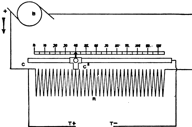
FIG. 105.—SHOWING REGULATION OF CURRENT BY RESISTANCE IN SHUNT.
