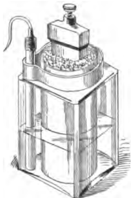
FIG. 28.—ORIGINAL LECLANCHÉ CELL.
