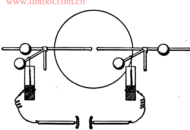
FIG. 99.—METHOD OF PRODUCING THE STATIC INDUCED CURRENT.
