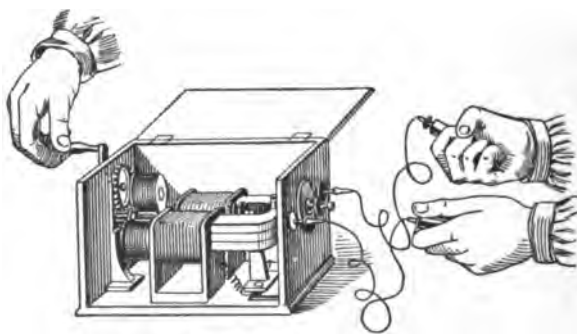
FIG. 138.—MAGNETO-ELECTRIC MACHINE.
