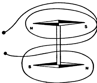
FIG. 52.—SHOWING THE METHOD OF WINDING COIL IN IMPROVED FORM OF ASTATIC GALVANOMETER.
