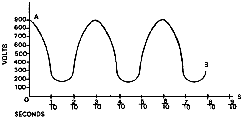
FIG. 76.—GRAPHIC REPRESENTATION OF A PULSATORY ELECTROMOTIVE FORCE.
