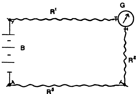
FIG. 35.—SHOWING A SIMPLE CIRCUIT CONTAINING THREE EQUAL RESISTANCE WIRES.
