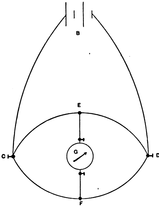
FIG. 65.—SHOWING METHOD OF DETERMINING UNKNOWN RESISTANCES BY THE WHEATSTONE BRIDGE.
