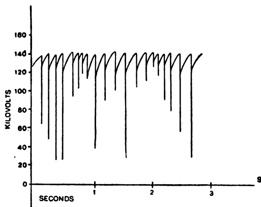
FIG. 85.—GRAPHIC REPRESENTATION OF A PULSATORY ELECTROMOTIVE FORCE.
