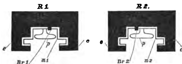
FIG. 103.—RIDERS OF COMBINED CELL SELECTOR.
