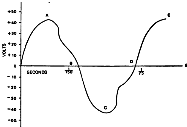
FIG. 82.—GRAPHIC REPRESENTATION OF A SYMMETRIC ELECTROMOTIVE FORCE.
