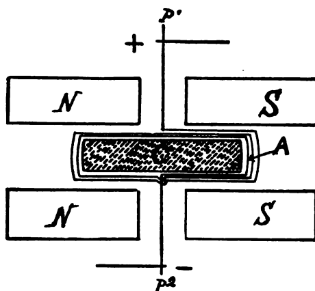
FIG. 119.—SHOWING TENSION SPRING OF MILLIAMPEREMETER.
