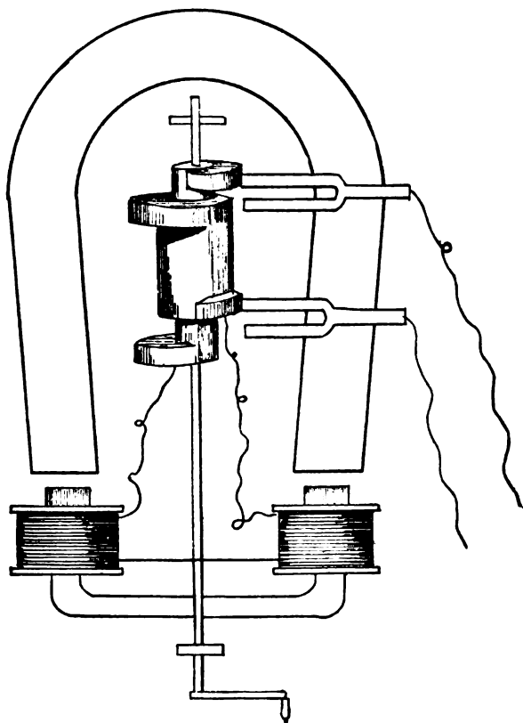
FIG. 70.—THE HORSESHOE INDUCTOR.
