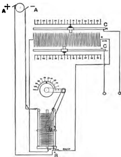
FIG. 137.—DIAGRAM SHOWING HOW THE CURRENT IS DERIVED FROM A DOUBLE SHUNT CIRCUIT.
