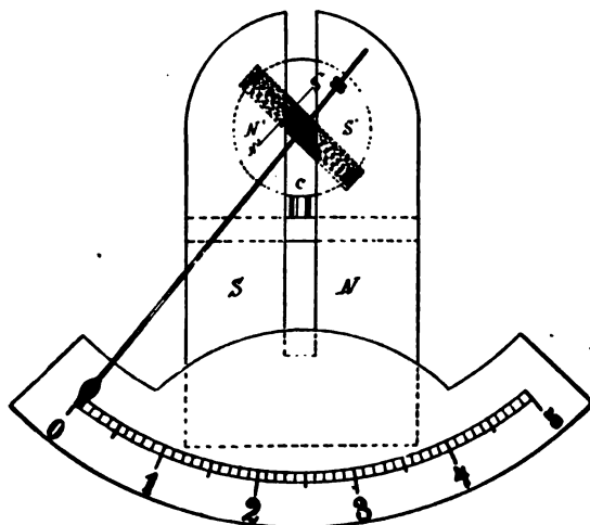
FIG. 118.—FRONT VIEW OF UPRIGHT MILLIAMPEREMETER.
