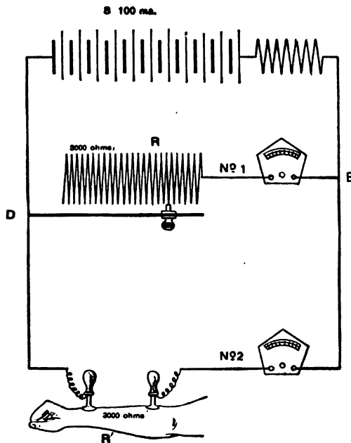
FIG. 41.—SHOWING THE PRINCIPLE OF THE SHUNT AS APPLIED TO ELECTRICITY.
