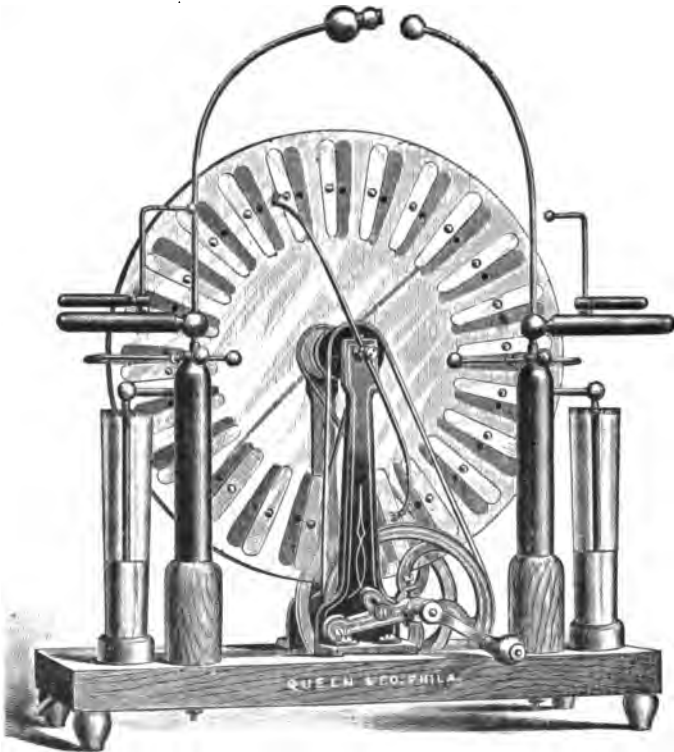
FIG. 15.—WIMSHURST MACHINE.
