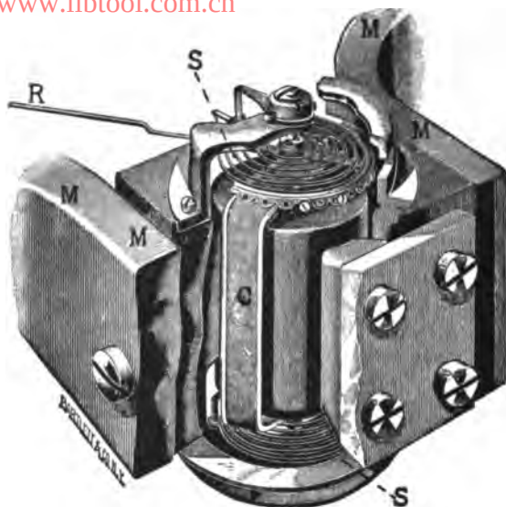
FIG. 58.—WESTON'S AMMETER, SHOWING WORKING PARTS.
