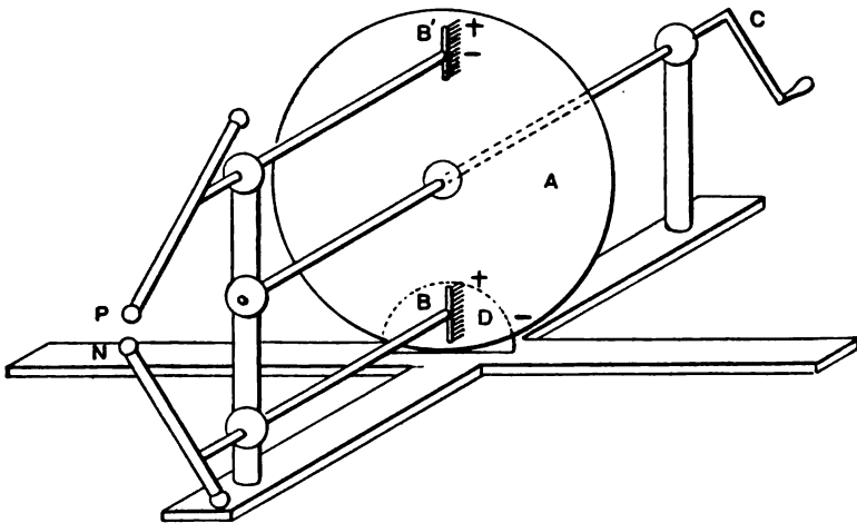
FIG. 14.—DIAGRAM SHOWING THE PRINCIPLE OF THE HOLTZ MACHINE.
