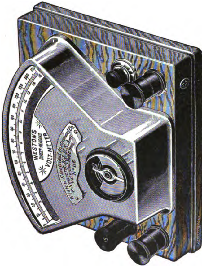
FIG. 61.—WESTON'S VOLTMETER.
