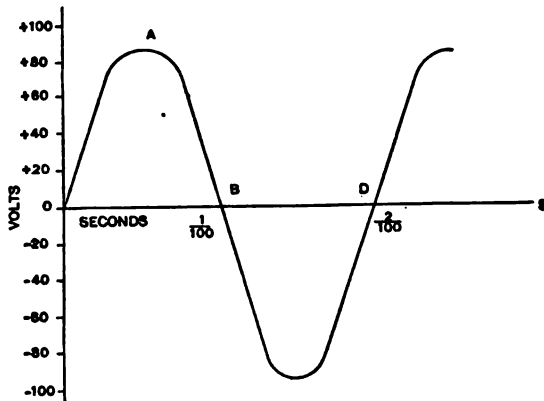
FIG. 79.—GRAPHIC REPRESENTATION OF A GRADUALLY ALTERNATING ELECTROMOTIVE FORCE.
