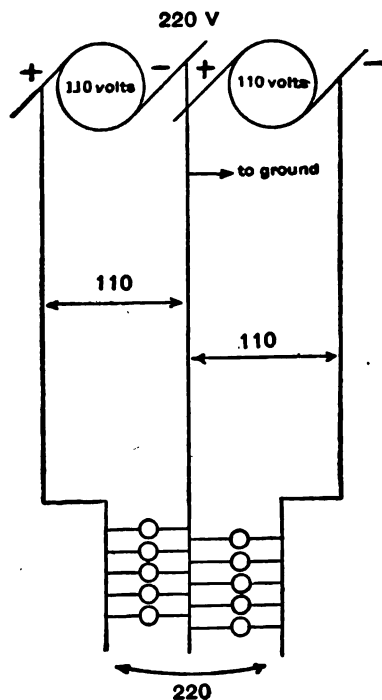
FIG. 134.—DIAGRAM SHOWING THE ARRANGEMENT OF WIRES IN THE 200 VOLT CIRCUIT.
