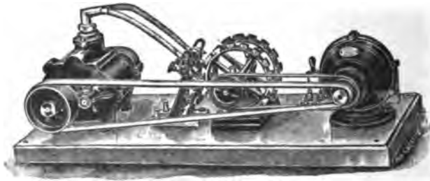
FIG. 156.—EDISON INSTANTANEOUS AIR-BREAK WHEEL.
