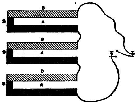
FIG. 72.—THERMOPILE.
