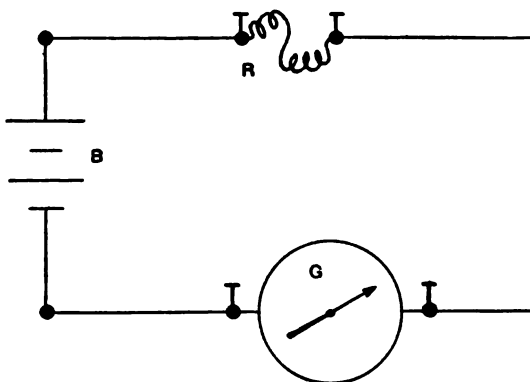
FIG. 64.—SHOWING METHOD OF DETERMINING UNKNOWN RESISTANCES BY SUBSTITUTION.
