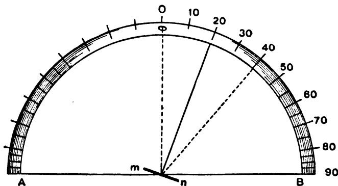
FIG. 54.—SHOWING COURSE OF DEFLECTED RAY ON SCALE OF MIRROR GALVANOMETER.
