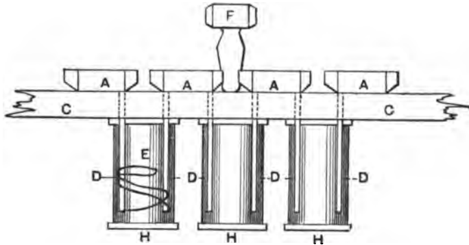
FIG. 62.—CONSTRUCTION OF RESISTANCE COILS.
