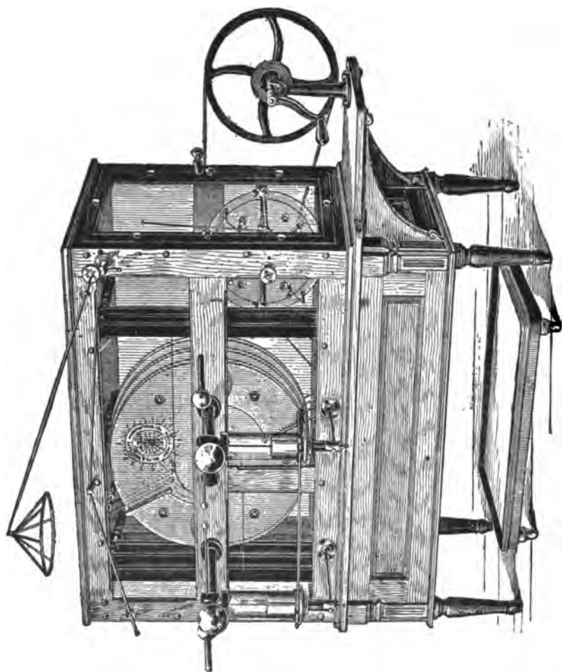
FIG. 90.—HOLTZ-TOEPLER MACHINE.—( Waite & Barlett, New York. )
