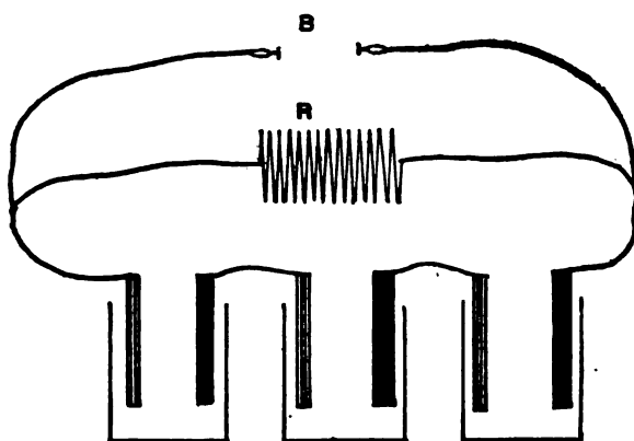
FIG. 115.—SHOWING A RHEOSTAT PLACED IN SHUNT.
