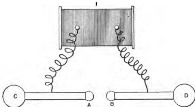
FIG. 88.—SCHEME OF HERZ'S INDUCTION COIL FOR PRODUCING HIGH FREQUENCY OSCILLATIONS.
