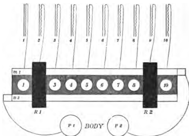
FIG. 102.—COMBINED CELL SELECTOR.
