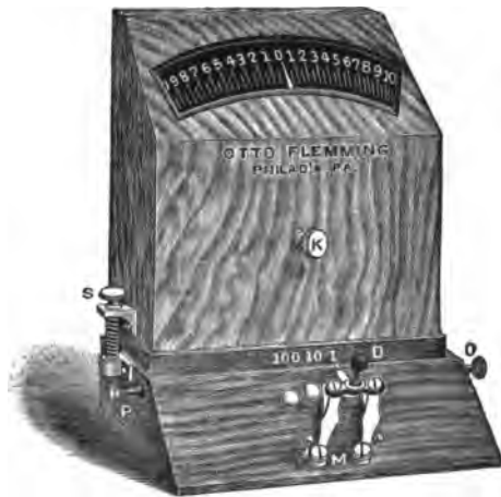
FIG. 120.—ANOTHER FORM OF UPRIGHT MILLIAMPEREMETER.
