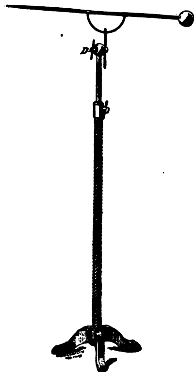
FIG. 98.—CONCENTRATOR AND STAND.
