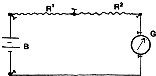
FIG. 37.—SHOWING A SIMPLE CIRCUIT CONTAINING TWO RESISTANCE WIRES IN SERIES.
