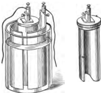
FIG. 25.—GROVE CELL.
