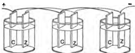
FIG. 43.—CELLS ARRANGED IN PARALLEL.
