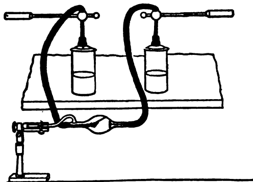
FIG. 155.—SHOWING THE ATTACHMENT OF X-RAY TUBE TO STATIC MACHINE.
