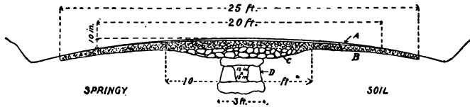
Fig. 6.—Type of road on a very wet foundation.
