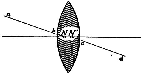
FIG. 4. Nodal Points of a Lens.
