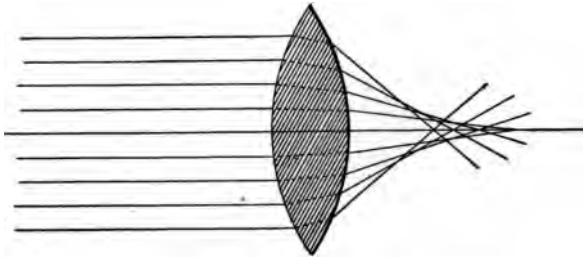
FIG. 16. Spherical Aberration.
