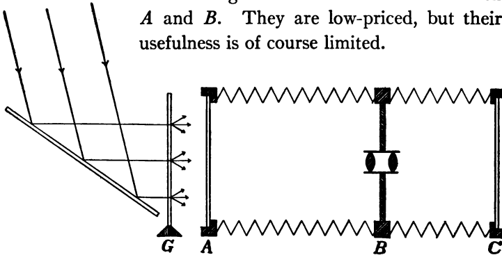
FIG. 77. Copying Camera.
