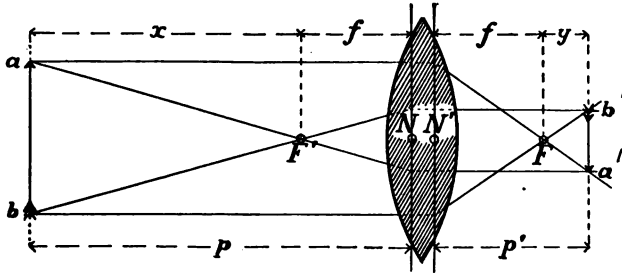
FIG. 7. Formation of an Image by a Lens.
