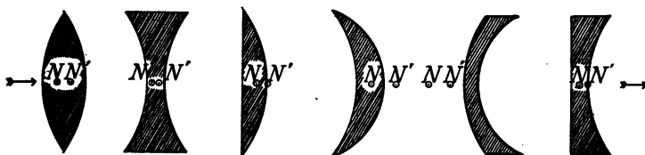
FIG. 5. Position of Nodal Points of Various Simple Lenses.
