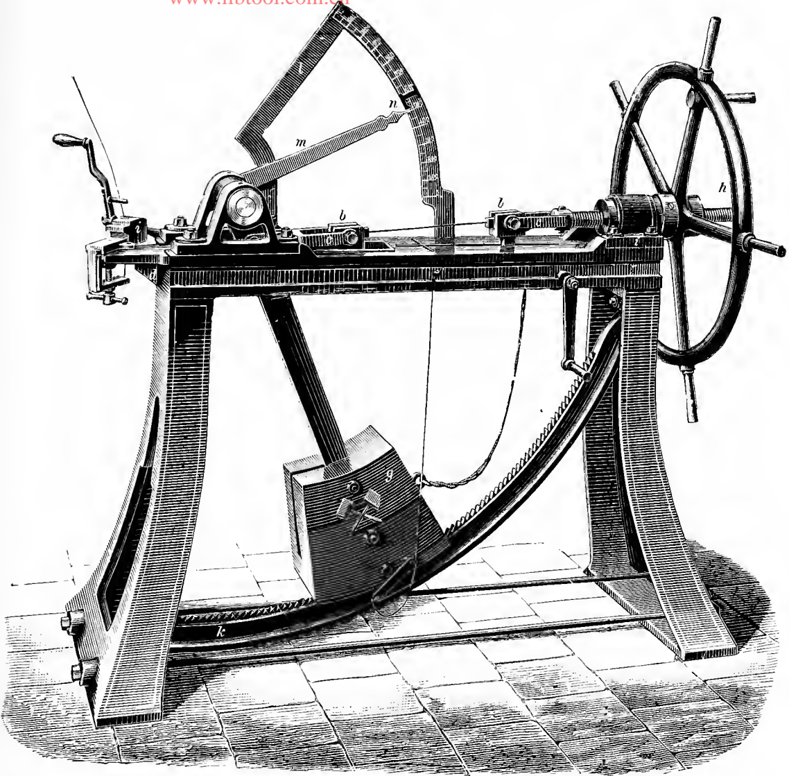
FIG. 13.— WIRE-TESTING MACHINE.
