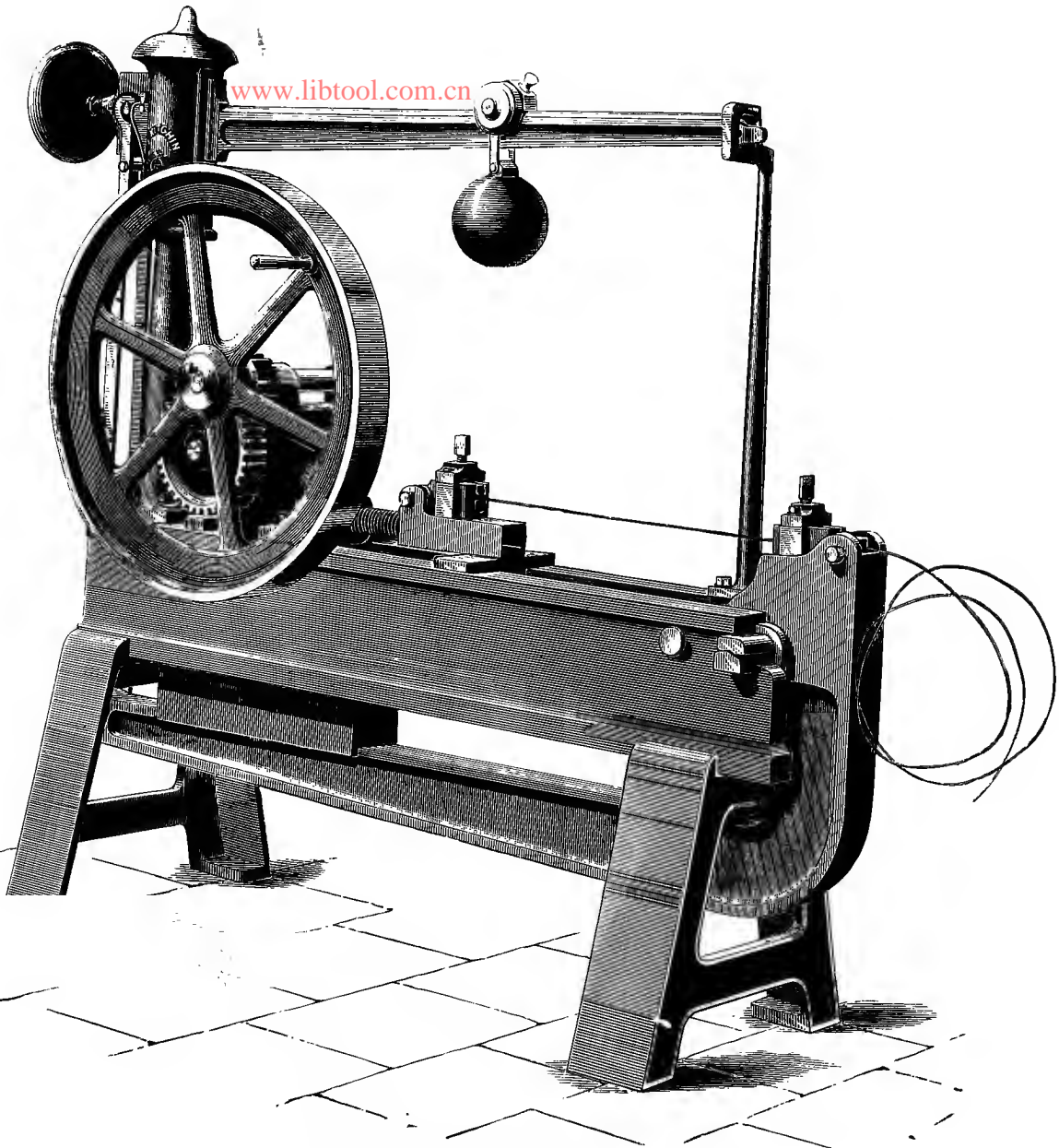
FIG. 19. KITCHIN'S WIRE-TESTING MACHINE.
