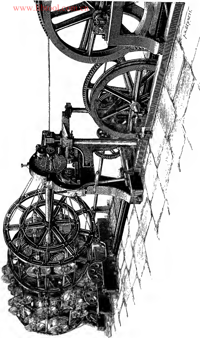
FIG. 1. 24-BOBBIN STRANDING MACHINE.
