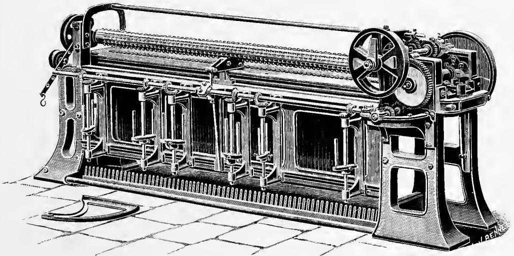
WILMOTT'S WIRE NETTING MACHINE.
