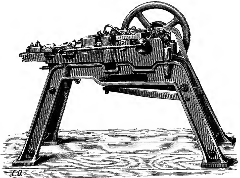
WIRE NAIL MACHINE AND PRESS.
