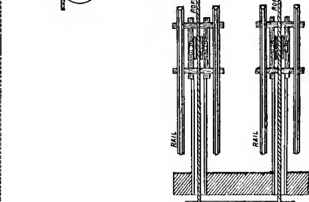
Terminal tension pulleys & carriages E: See Fig. 3.
