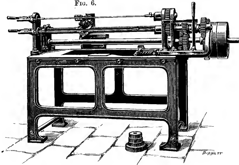
BOND'S WIRE NETTING AND SPRING COILING MACHINES
