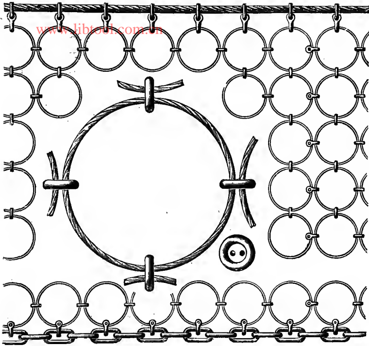
FIG. 13. TORPEDO NETTING.
