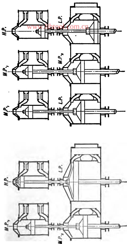
FIG. 8C. Quadruple Expansion Engines.
