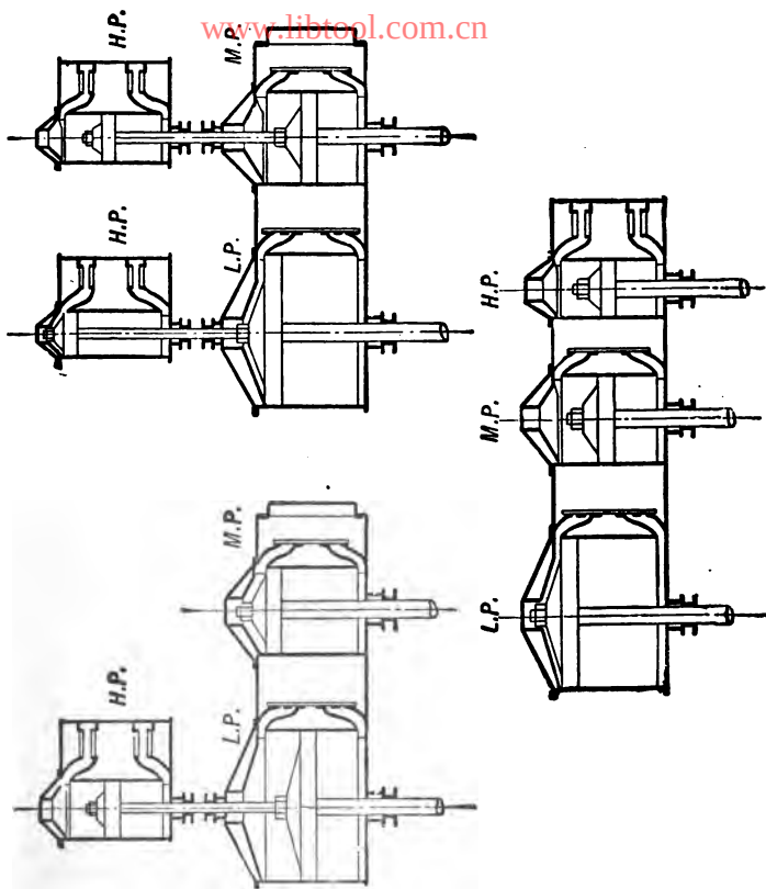
FIG. 3 Triple Expansion Engines.
