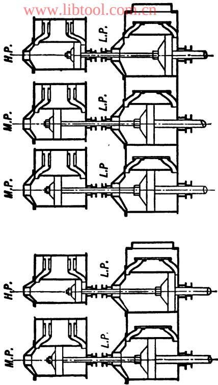
FIG. 38. Triple Expansion Engines.
