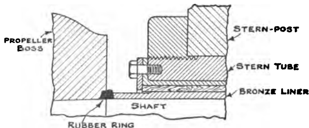
FIG. 20.—Shows an arrangement of after-end of the stern tube, shaft, and screw boss as generally adopted.
