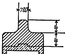
Cast-steel Strap with Bronze liner.
