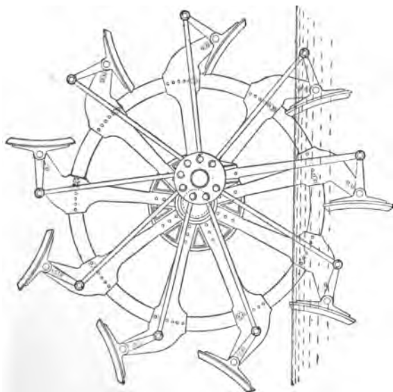
FIG. 43.—Paddle-Wheel with Steel Floats and no Outer Rim.
