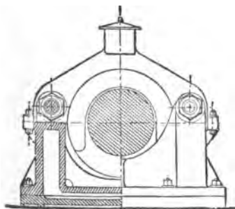
FIG. 22.—Thrust Block.
