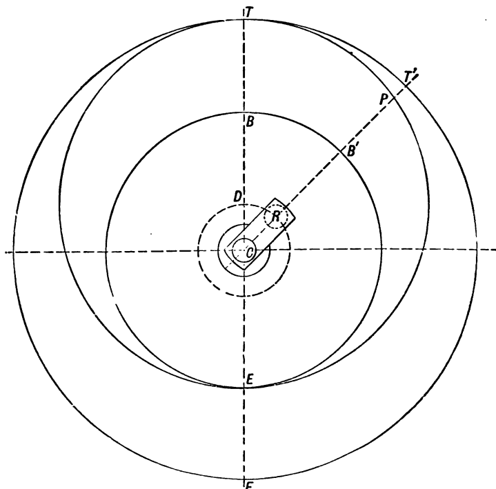
FIG. 28.—Diagram of the Piston Path.
