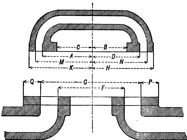
FIG. 27.—Proportions of a Trick Valve.
