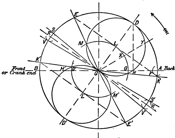
FIG. 29.—Zeuner's Diagram for the Common Valve Motion.
