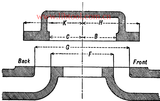
FIG. 26.—Proportions of a Common Valve.
