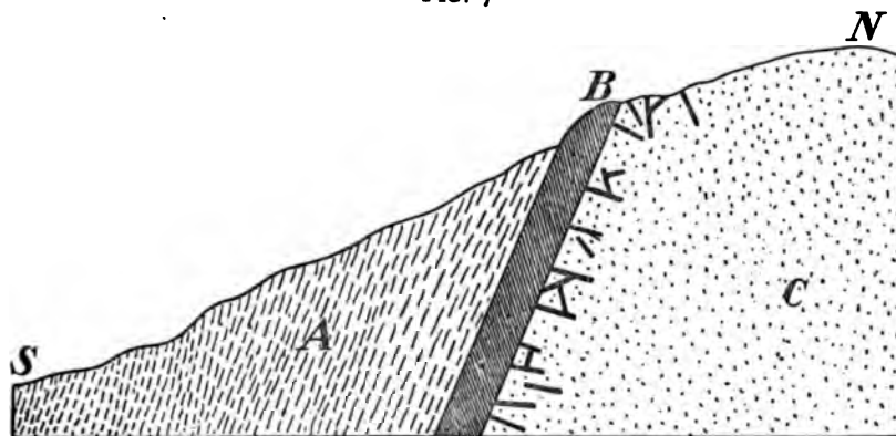
Section through the Layton Mine, Georgia, showing the Mode of Occurrence of the Iron and Manganese Deposit (Modified from Penrose). A. Manganese-bearing Clay containing Ore in nodules and layers. B. Iron and Manganese Ore stratum. C. Sandstone. Horizontal and Vertical Scale: 1 inch=50 feet.
