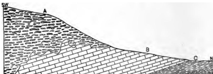
Section through the Barnsley Tract, Georgia, Showing a Manganese-bearing Chert Belt (Modified from Penrose). A. Chert and Cherty Limestone. B. Limestone. C. Shale.
