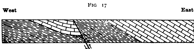
Section across Valley, \frac{3}{4} mile South of Lindale, Floyd County, Georgia.
