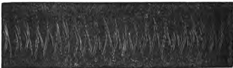
Trace of the median course of the wing of the Macroglossa galium , (Bedstraw sphynx-moth.)
