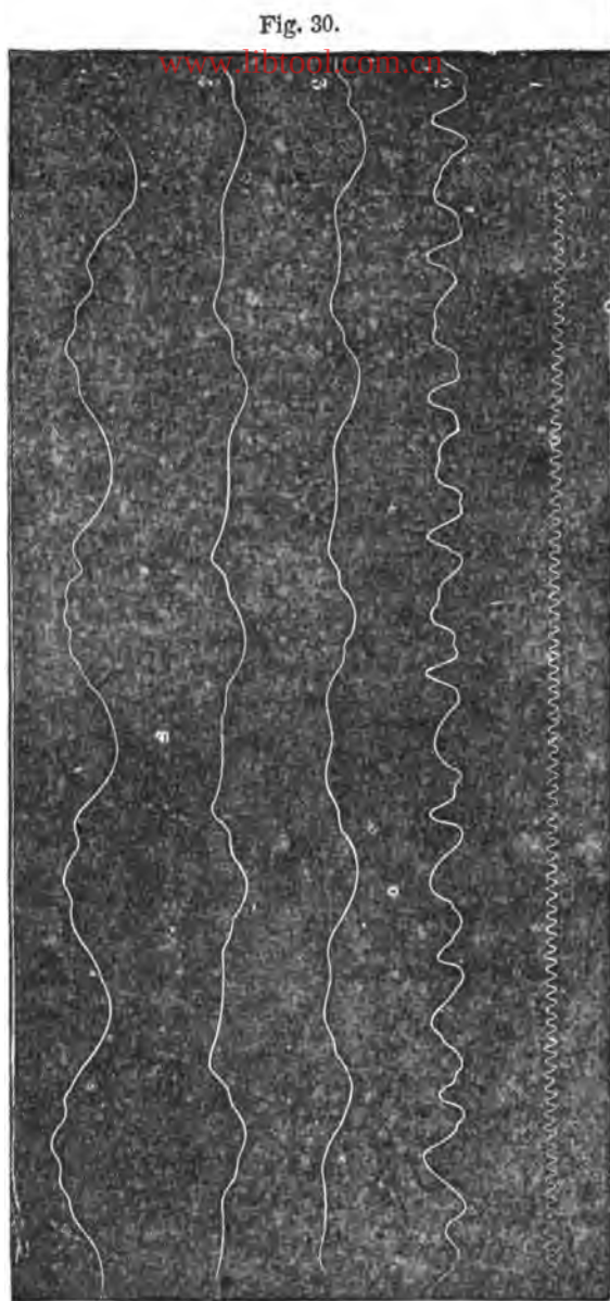
Fig. 30. Line 1. Chronographic trace of a tuning-fork, vibrating 100 times a second; 2. Vertical oscillations of the wild duck during flight. 3. Oscillations of the hen-hawk. 4. Of the screech-owl; and 5, of the harrier.
