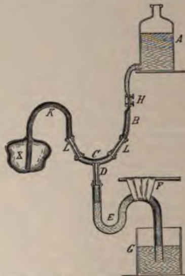
FIG. 384.—Keen's modification of Cathcart's siphonage apparatus: X , cavity to be drained; A , reservoir; K , tube from cavity; B , tube from reservoir; H , clamp on tube from reservoir; L , L , D , glass tubes; C , rubber tube connecting cavity-drain with reservoir-drain; E , S-shaped rubber tube maintained in shape by hooking up at F ; G , vessel containing antiseptic fluid.
