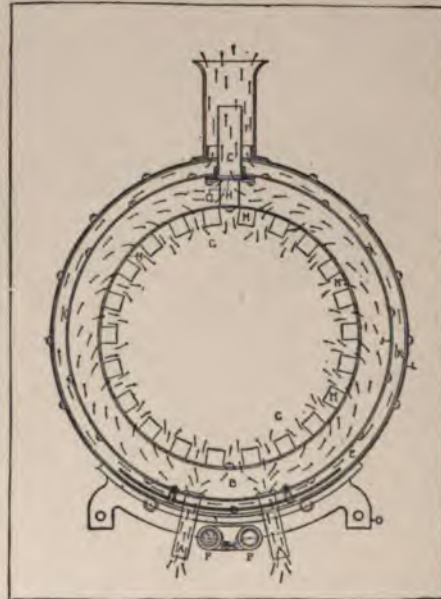
FIG. 165.—Cross-section of Sprague hot dry-air apparatus: A, A, air intakes; n, circulating air space; H, jacketed space for products of combustion; G, treatment-chamber; M, M, cork ribs; N, N, perforations admitting heated air; O, base holding apparatus; P, R, gas-burners.
