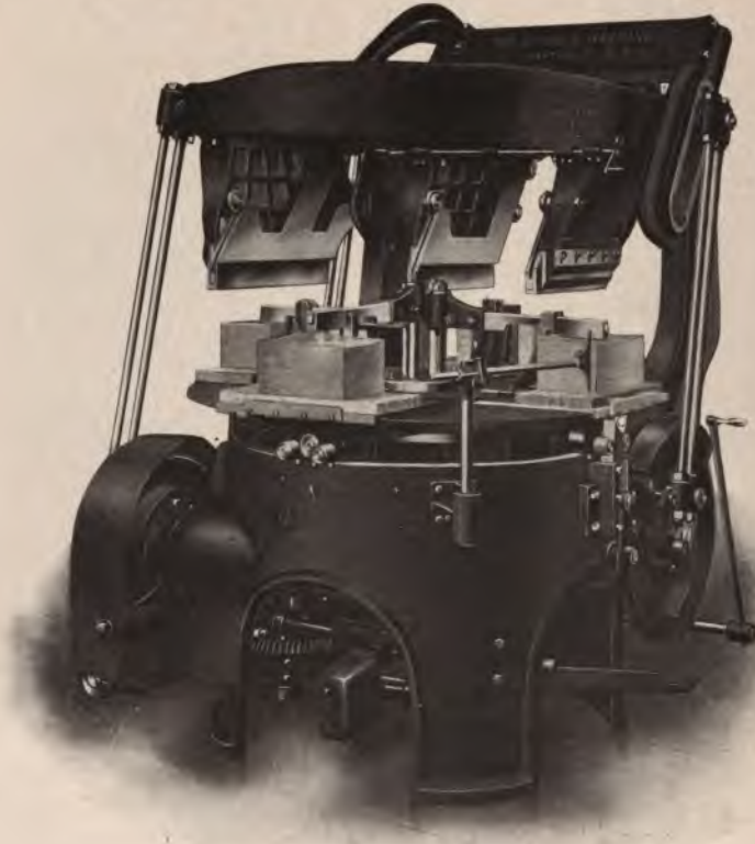
Seybold Continuous Trimmer.
