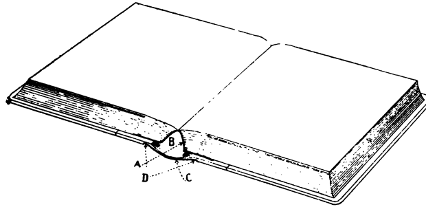
A — Flesher leather. B — Manila paper. C — Leather back. D — Joint.
