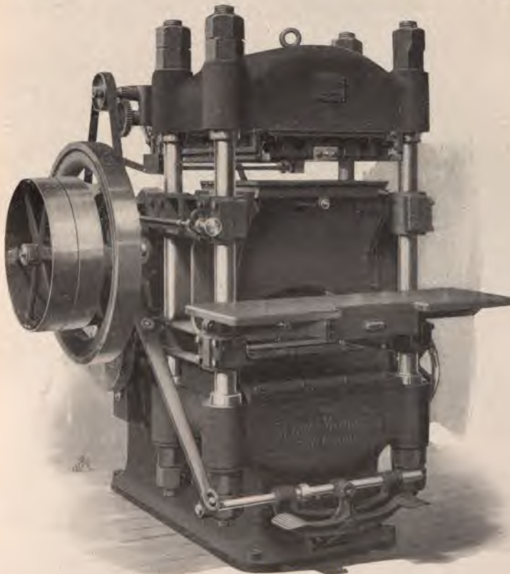
Seybold Inking and Stamping Press. (263)
