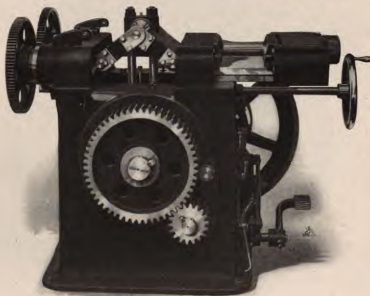
Seybold Book Compressor Stripped, Showing Toggles and Gearing.
