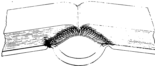
Spring-back Guard-sewed Book, Termed Patent Back.
