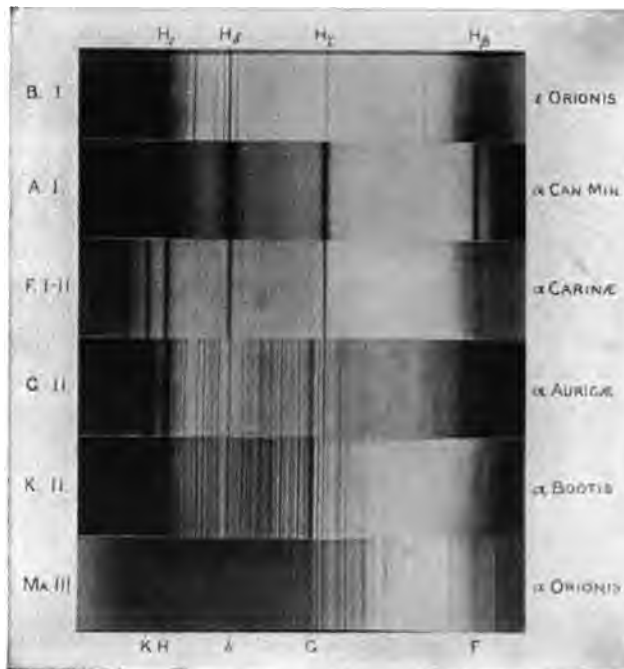
FIG. 21.—TYPICAL SPECTRA
