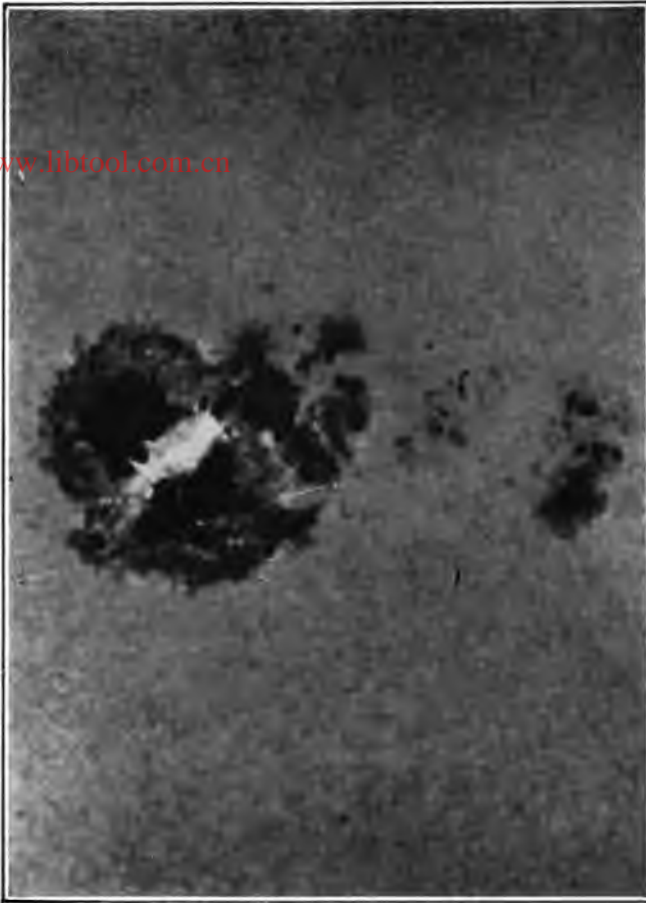
Yerkes Observatory.
