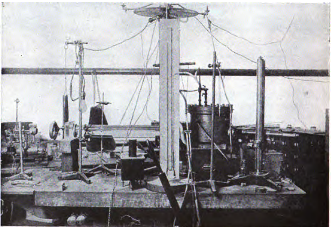
PROFESSOR R. A. MILLIKAN'S APPARATUS FOR COUNTING ELECTRONS
