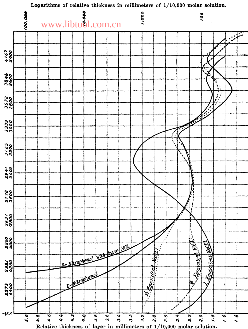
FIG. 3.—O-nitrophenol; O-nitrophenol with trace HCl—upper full curves. O-nitrophenol with 1/10 equivalent of sodium ethoxide—dot curve. O-nitrophenol with \frac{1}{2} equivalent of sodium ethoxide—dash curve. O-nitrophenol with 1 equivalent of sodium ethoxide—lower full curve.
