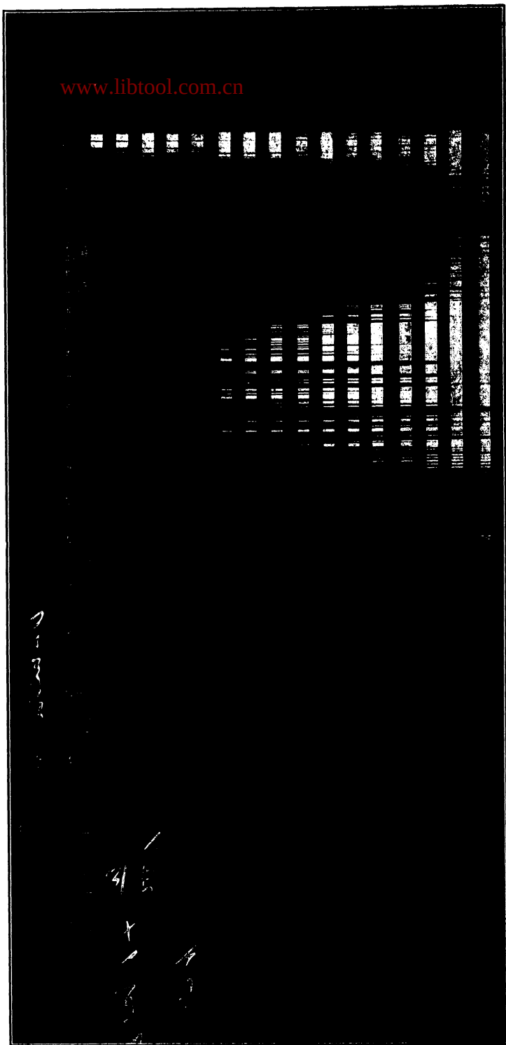
PLATE II. O-NITROPHENOL WITH 1 EQUIVALENT OF SODIUM ETHOXIDE. 1/1000 MOLAR SOLUTION. THICKNESS OF LAYER, 32 TO 2 MILLIMETERS.
