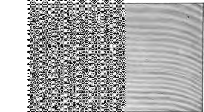
structure in layers. (Natural size.)
