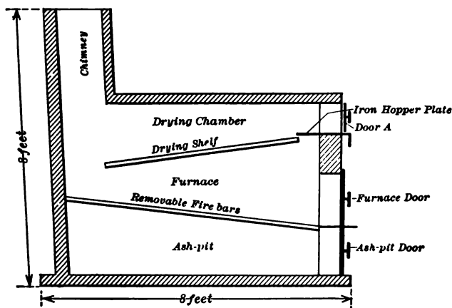
FIG. 29.—Fixed incinerator, with drying shelf. The damp refuse is pushed through door A into the drying chamber, where it is exposed to the heat of the furnace. When dry the refuse is pushed over the edge of the shelf into the furnace. The "drying shelf" is made of perforated iron. This pattern may be used for incineration of faeces.
