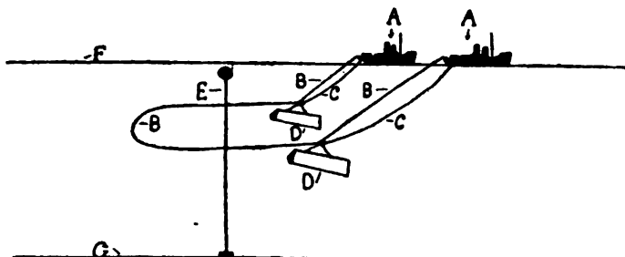
FIG. 25.—Diagram showing the form of apparatus principally used by British minesweepers. AA. Sweeping vessels. BB. Sweep-wire. CC. Wires holding kites. DD. Kites which hold sweep-wire at correct depth below the surface by their "kite-like" action when being towed through the water. E. Mine and mooring. F. Surface of the sea. G. Sea-bed.
