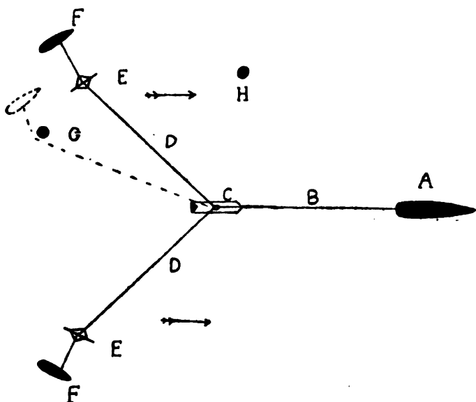
FIG. 26.—Diagrammatic sketch showing principal parts of a single-ship sweep. A. Towing vessel. B. Tail wire. C. Kite holding sweep-wires D at correct depth below the surface. D . Light sweep-wires held at an angle by spars E and surface hydroplane floats F . The dotted lines show how either arm of the sweep swing towards the centre line when exposed to the pull of a mine. This movement of the hydroplane floats indicates to those on board the sweeping vessel that a mine has been caught. The mine H slides down the sweep-wire until the mooring is cut at G , and the mine floats freely to the surface.
