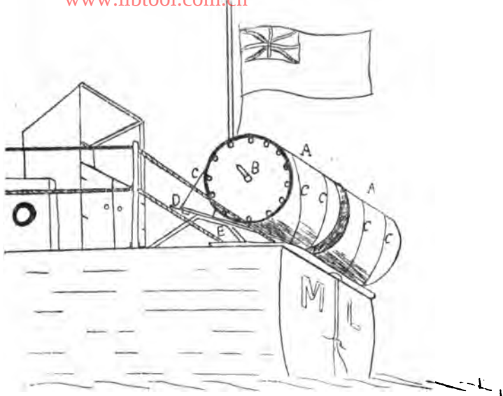
FIG 9.—Diagram showing how depth charges are carried on the stern of a motor launch. AA . Depth charges, each containing 300 lb. of high explosive. B . Hydrostatic device by means of which the charge can be made to explode when it has sunk from the surface to a depth of 40 or 80 feet, and by which it is rendered comparatively safe while on deck. C . Slings holding charges in place on inclined platform. D . Greased bolts which, on being pulled out, allow wire slings to fly free and depth charge to roll into the sea. Depth charges can only be released from vessels under way, otherwise the explosion which occurs a few seconds after release damages surface vessel.
