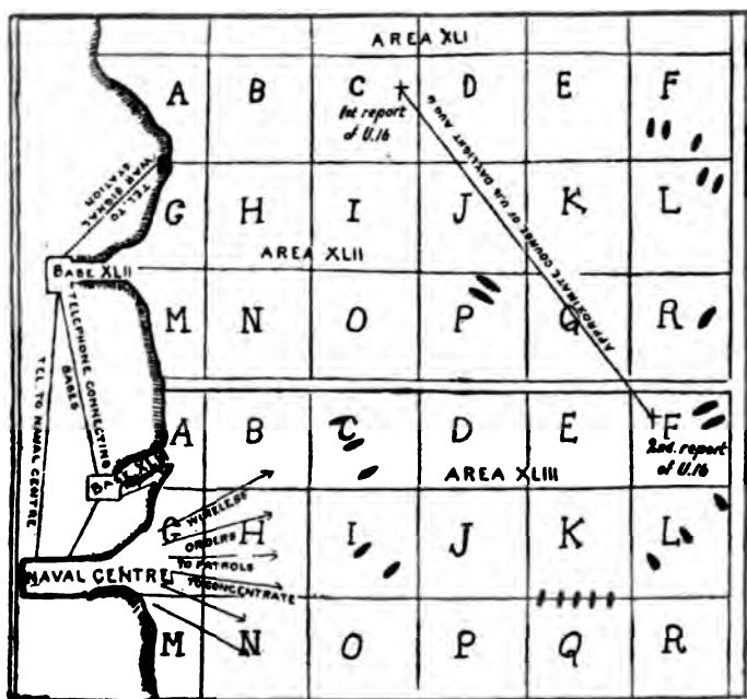
FIG. 20.—Diagram showing division of sea into anti-submarine patrol areas.
