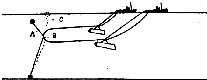
FIG. 27.—Diagram showing mine mooring being cut by sweep-wire. A. Mine-mooring wire. B. Hard and cutting face of sweep-wire. The dotted lines C show how the mine floats to the surface by its own buoyancy when the mooring wire holding it down has been cut.
