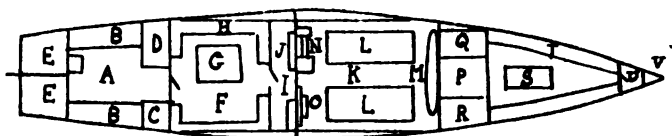
FIG. 2.—Plan of armed motor launch, showing internal arrangements. A. Officers' sleeping cabin. B.B. Bunks. C. Cupboard. D. Lavatory. E.E. Stern petrol tanks. F. Wardroom. G. Table. H. Settee. I. Galley. J. Petrol stove. K. Engine-room. L.L. Main engines. M. Compressed air reservoirs. N. Auxiliary petrol engine driving dynamo, bilge pumps, fire pumps and air compressor. O. Electric storage batteries, switchboard and electrical starting arrangements for auxiliary engine. P. Chart-room with petrol tanks below. Q. Magazine. R. Fresh-water tanks. S. Forecastle. T. Bunks for crew. U. Forecastle lavatory. V. Watertight forepeak.
