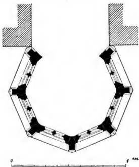
Figur 2. Grundriss.
