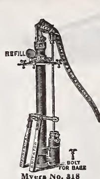
Myers No. 318
