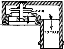
FIG. 155.—Morey's Trap Attachment.
