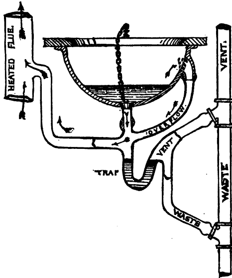
FIG. 258.—Ventilation of House-side of Trap.
