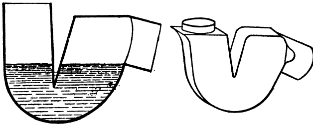
FIG. 93.—Hellyer's Mansion Trap.
