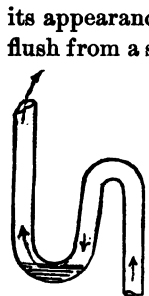
FIG. 18.—Water seal of S-trap lost by siphonage or evaporation.
