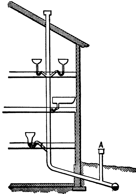
FIG. 24.—Soil pipe extended full size, and provided with foot-ventilation; each fixture in the house trapped by a trap, but no trap on the main drain.
