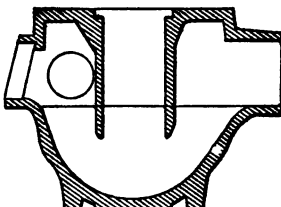
FIG. 77.—McLandsborough's Trap.
