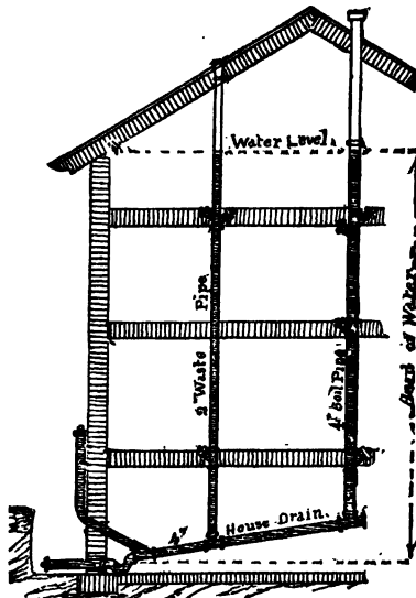
FIG. 22.—Sketch showing method of applying the water pressure test.
