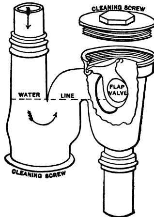
FIG. 150.—Barrett's Trap.
