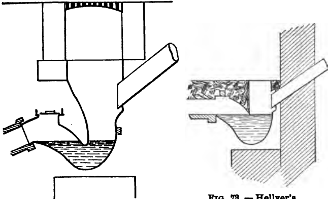
FIG. 72.—Hellyer's Soil-pipe Disconnector. FIG. 73.—Hellyer's Drain Interceptor. "Combina- tion Soil Pipe Trap." Fig. 73 shows Mr. Hellyer's Drain Interceptor Trap.
