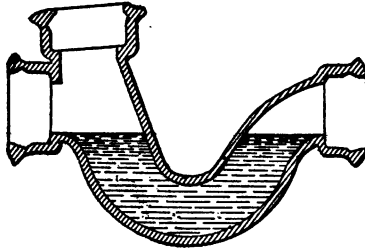
FIG. 46—Durham Trap, with fresh air inlet only.
