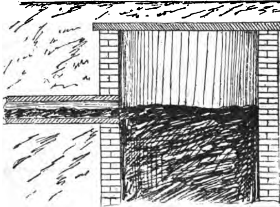
FIG. 179.—House drain delivering into a filled cesspool.
