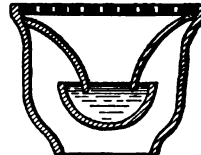
FIG. 100.—Antill's Trap. FIG. 101.—Jennings' Improved Bell-Trap.
