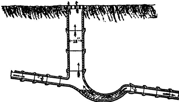
FIG. 54—Disconnecting Trap.
