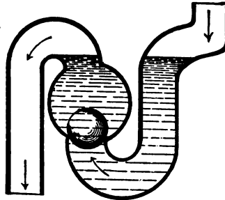
FIG. 143.—Turner's Trap.
