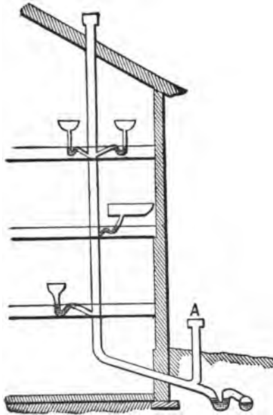
FIG. 36.—House drain trapped by a running trap; fresh air pipe on house side of trap; trap under each fixture; soil pipe extended full size above the roof.
