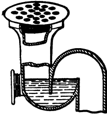
FIG. 101a.—Tye & Andrews' Sink Trap.
