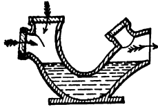
FIG. 51.—Suitable Stoneware Trap for house drains.
