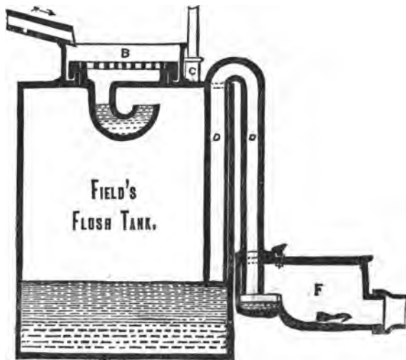
FIG. 278.—Field's Flush-tank.
