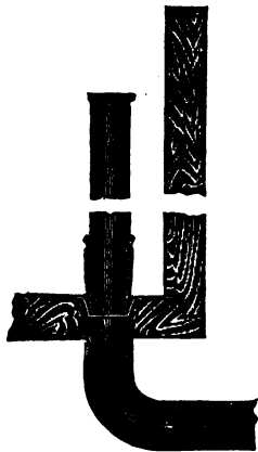
FIG. 228—Standing Overflow.
