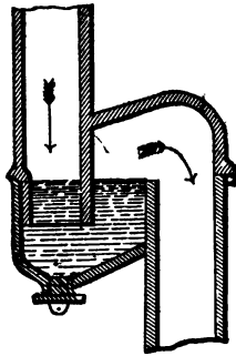
FIG. 92.—Adoo's Patent Stench Trap.
