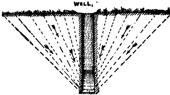
FIG. 180.—Cone of filtration.
