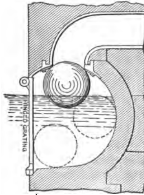
FIG. 87.—Jennings' Improved Tidal Valve.
