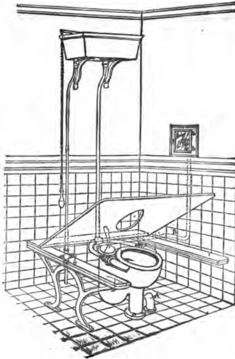
FIG. 251.—Brighton water closet seat.
