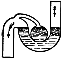
FIG. 156.—W. Scarborough's Trap.
