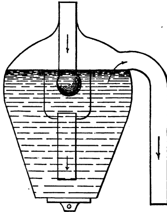
FIG. 138.—Knight's Trap.
