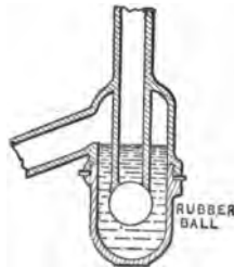
FIG. 130.—Bower's Trap in section.
