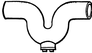
FIG. 111.—Du Bois' Running Trap.
