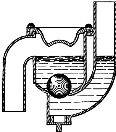
FIG. 141.—Garland Trap.
