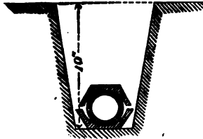
FIG. 274.—Cross section through a trench, with absorption drains.
