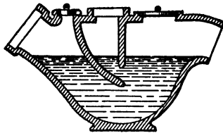
FIG. 66.—Stiff's "Interceptor" Sewer Air Trap.
