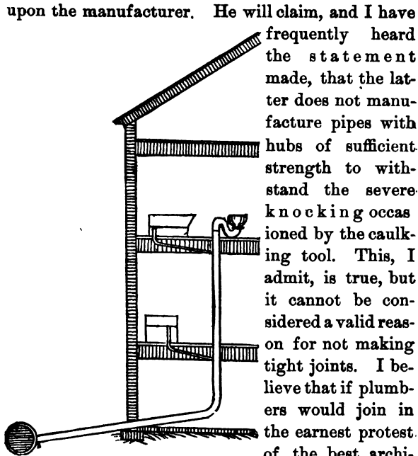
FIG. 23.—Soil pipe from water closet trap to the sewer without extension through the roof. No fresh air pipe and no trap on main drain.
