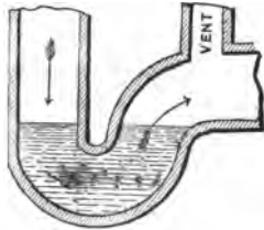
FIG. 96.—Lead P or \frac{1}{4} S-Trap, with vent attached.
