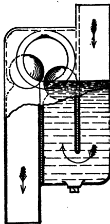
FIG. 154.—Randolph's Trap.
