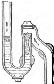
FIG. 139.—Waring Trap.
