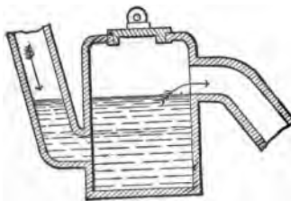
FIG. 115.—Boston Round Trap.
