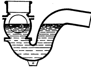
FIG. 137.—Putzrath's Back-Pressure Valve.
