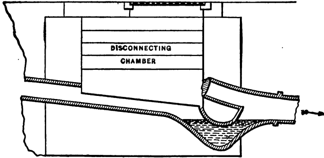
FIG. 52.—Disconnecting Trap.
