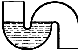
FIG. 98.—Lead S-Trap.
