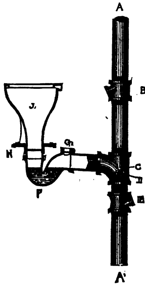
Fig. 182.—Soil Pipe with branch supporting a hopper-closet, with iron trap below the floor.
