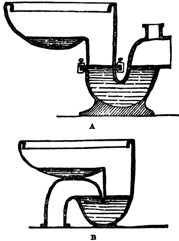
FIGS. 236a and b.—Author's Suggestion for Improving Washout Closet.
