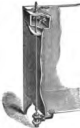
FIG. 224.—Boston Waste Cook.
