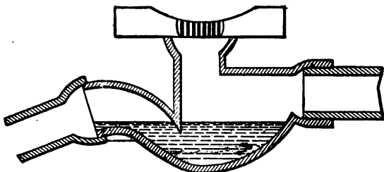
FIG. 59—Molesworth's Trap.
