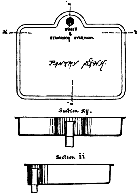
FIG. 208.—Pantry Sink with standing overflow.
