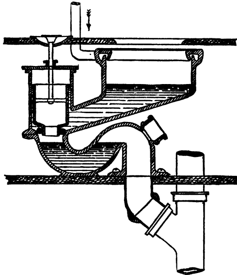
FIG. 13.—Plunger Closet.
