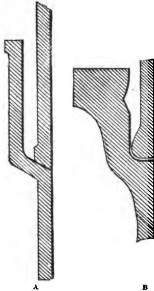
FIG. 21.—Sketch showing comparative strength of hubs of plumbers' pipe and gas pipe. A—Plumbers' pipe. B.—Gas pipe.
