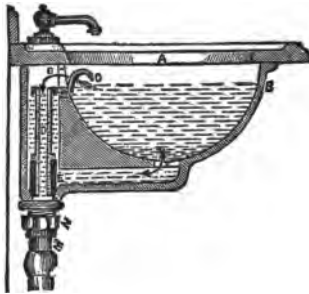
FIG. 215.—Bennor's Waste Valve.
