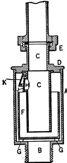
FIG. 120.—Pletsch's Stench Trap.
