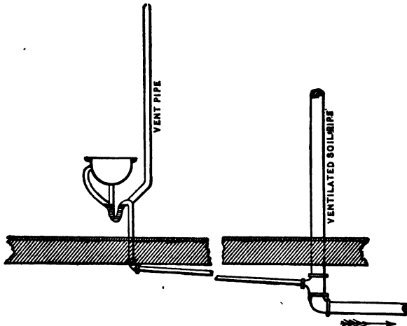
FIG. 168.—S-trap vented to prevent a long dead end in the waste pipe.
