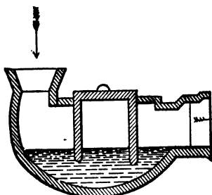
FIG. 76.—Cottam's Trap.
