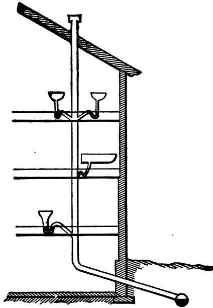
FIG. 38.—Fixtures trapped and soil pipe extended full size above the roof, but house drain left in direct connection with sewer or cesspool.
